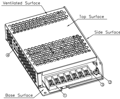
Figure 7. PMT-24V150W2BA System Design [13]
