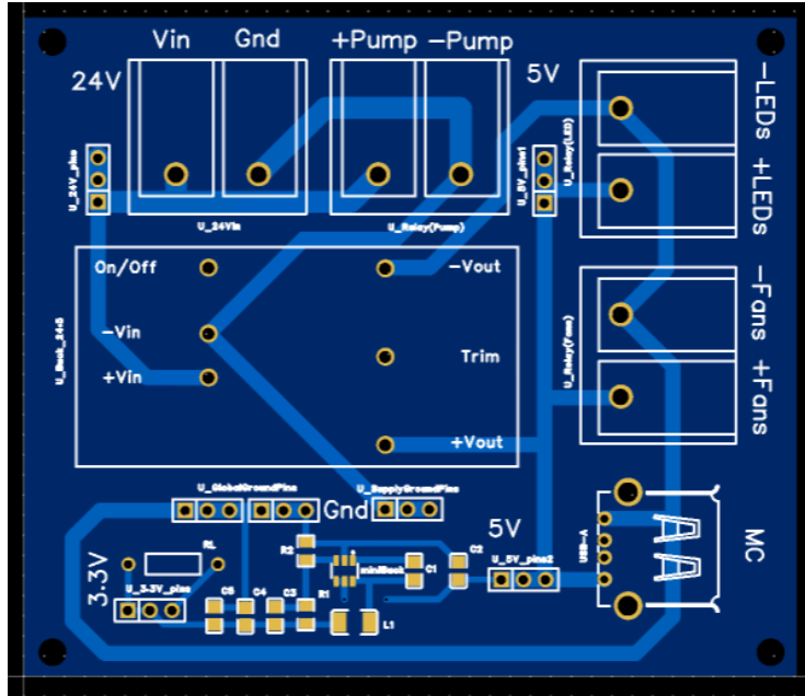
Figure 11. PCB Layout via EasyEDA
