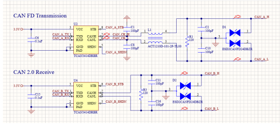
Fig. 9: CAN Transceivers
