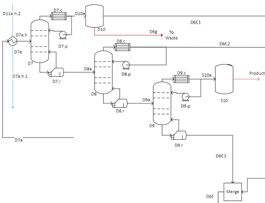
Figure 21: Process Flow Diagram of the Distillation Cascade
