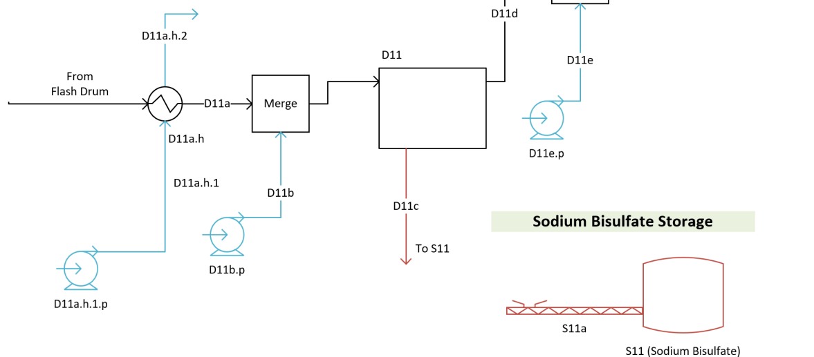
Figure 17: Process Flow Diagram for Sedimentation Tank
