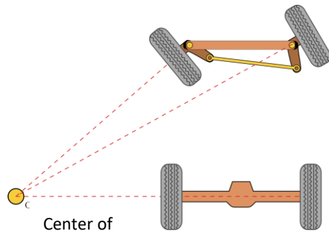
Figure 3. Variable wheel turning radius when rounding a turn
