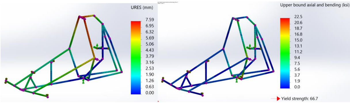
Figure 14. Side load case resultant displacement and upper bound stress plots (final design)
