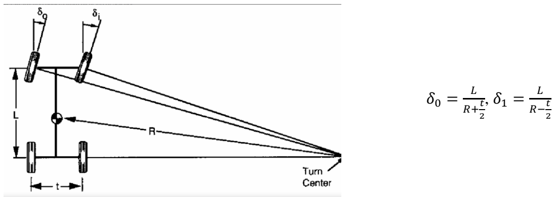
Figure 20. (left) Showing the geometric relationship that creates the turn center based on tire angles, (right) Equations that relate the tire angles with the turning radius of a vehicle
