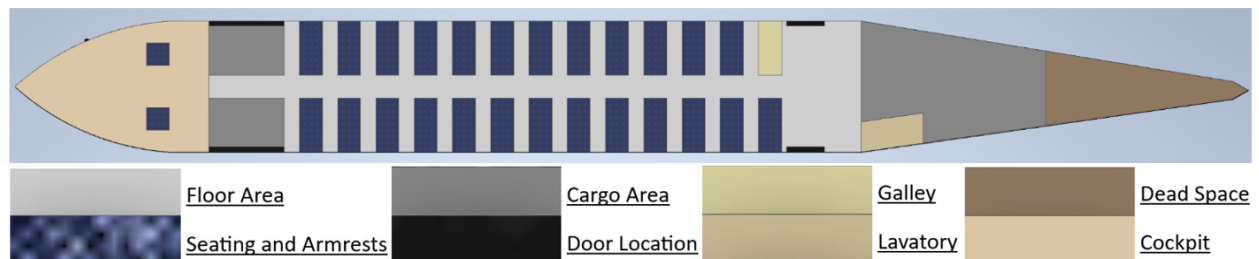
Figure V-2. General Layout of the Passenger Cabin and Cargo Storage Areas in Inches
