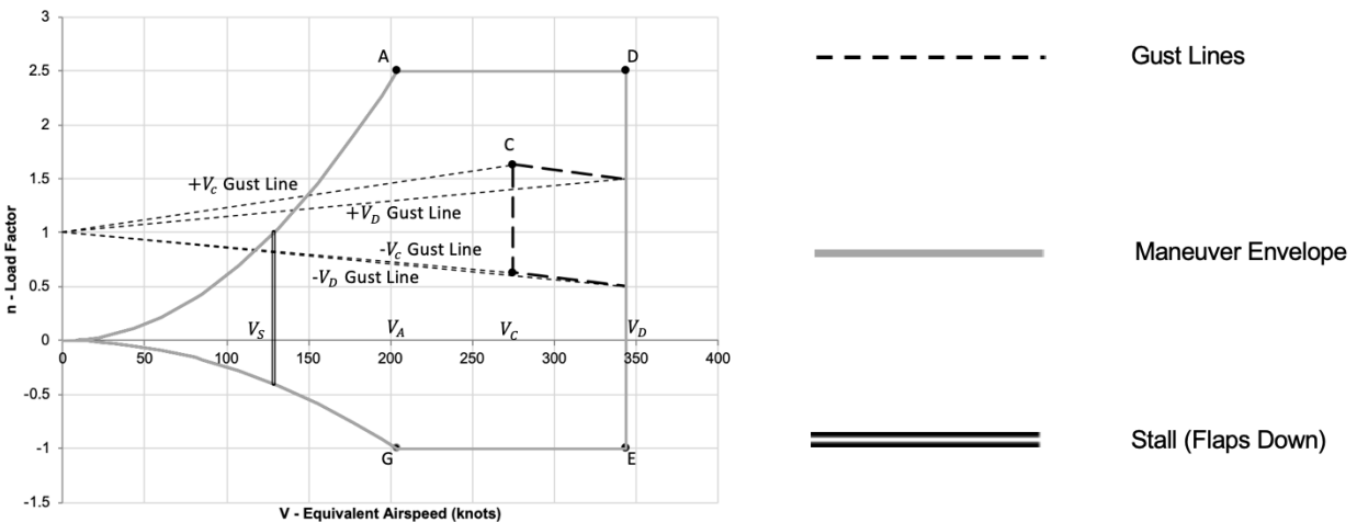
Figure XI-1. V-N Diagram
