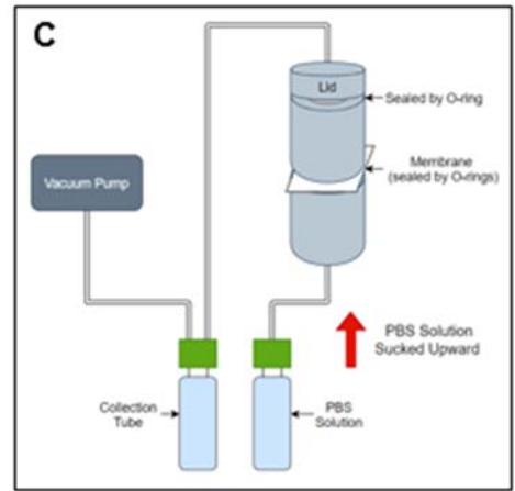
Fig. 4. Updated Design Schematic for the Encapsulation Device. In this updated version of the initial design schematic, the three step process for encapsulating mNSCs with a single layer coating is described (A,B,C). For any additional layers, the three steps should be repeated.
