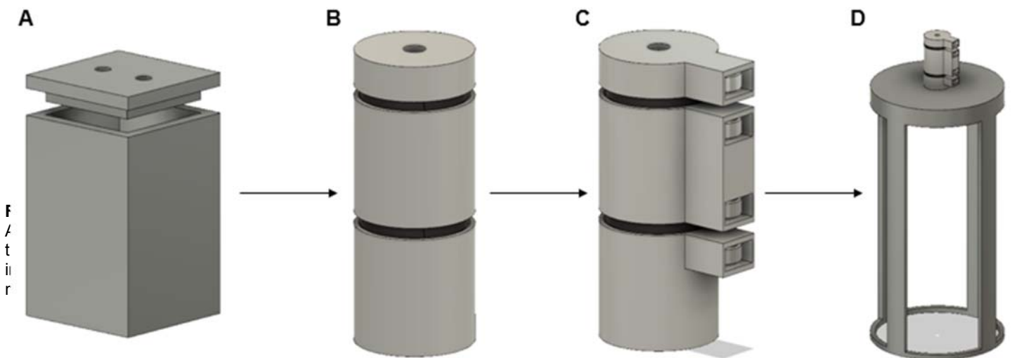
Fig. 5. Iterations of the Device Design. The four iterations of the CAD design for the device prototype are illustrated including: the initial design (A), the updated design (B), the updated design with magnetic clasps (C), and a support stand to hold the final prototype design (D).
