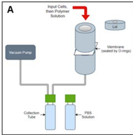
Fig. 4. Updated Design Schematic for the Encapsulation Device. In this updated version of the initial design schematic, the three step process for encapsulating mNSCs with a single layer coating is described (A,B,C). For any additional layers, the three steps should be repeated.
