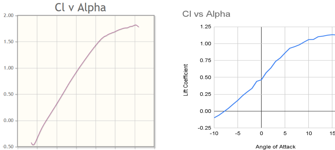
Figure 7: (Left) C_l vs Alpha curve at Re = 500,000 from Airfoiltools.com and (Right) C_l vs Alpha from experimental data
