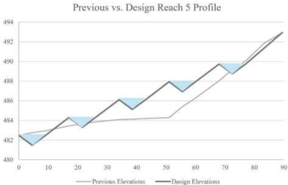
Reach 5 Profile View of Existing vs Proposed Elevations
