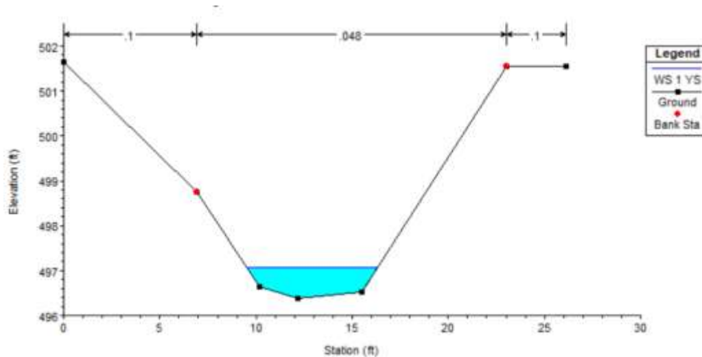
Figure 4-4. Cross Sectional View in Reach 3 of Surface Water Level from 1-Year Storm
