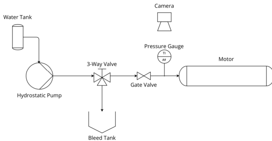
Figure 81. Schematic for Hydrostatic Test
