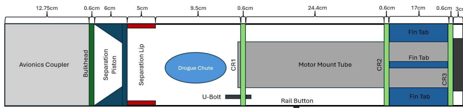
Figure 62. Aft Body Section
