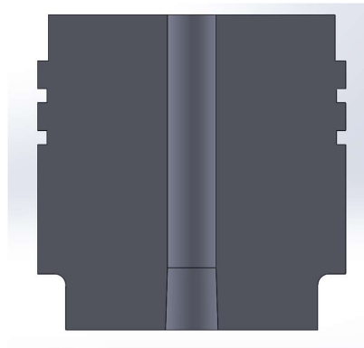
Figure 51. Hydrostatic Nozzle
