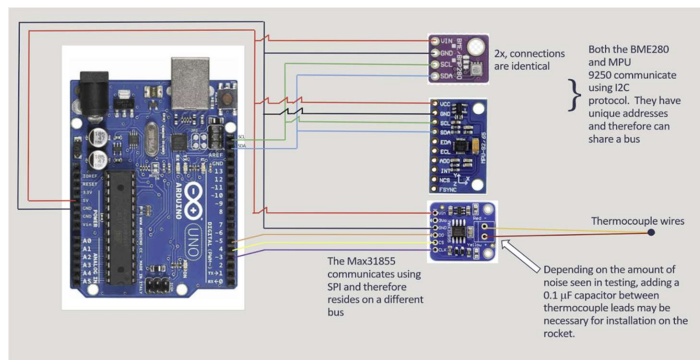
Figure 68. The circuit diagram for our first prototype.
