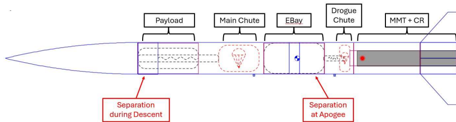
Figure 1. Labeled Final Open Rocket Model
