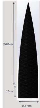
Figure 3. Final ogive nosecone design and dimensions.
