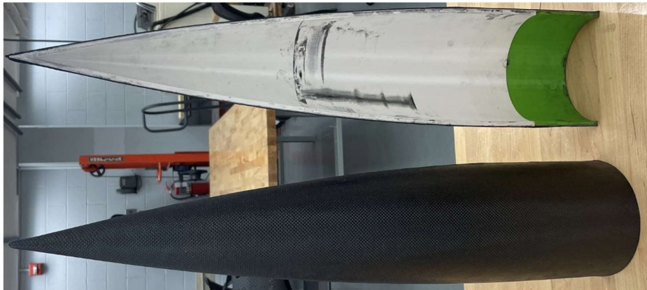
Figure 57. After 3 layers of CFRP wet layup
