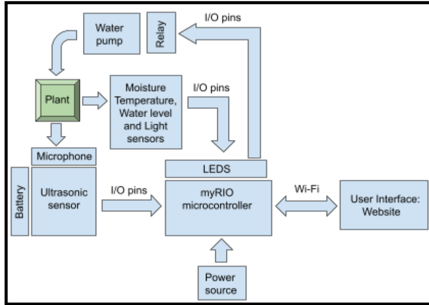
Figure 5: Block diagram of full system
