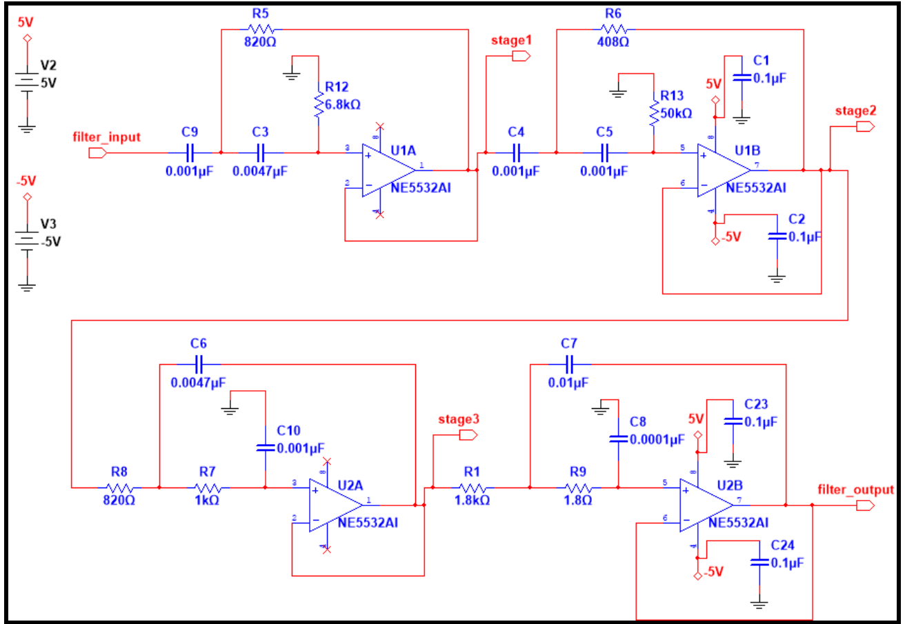
Figure 2: Filter Design
