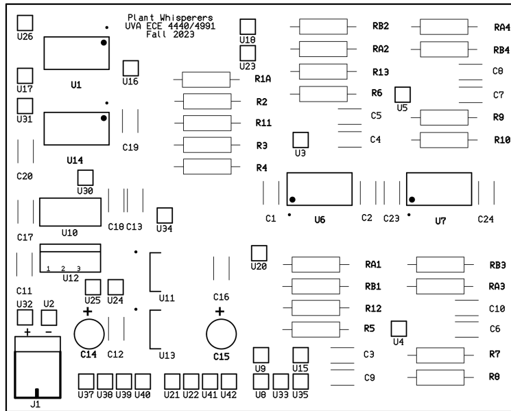
Figure 4: Final PCB Layout
