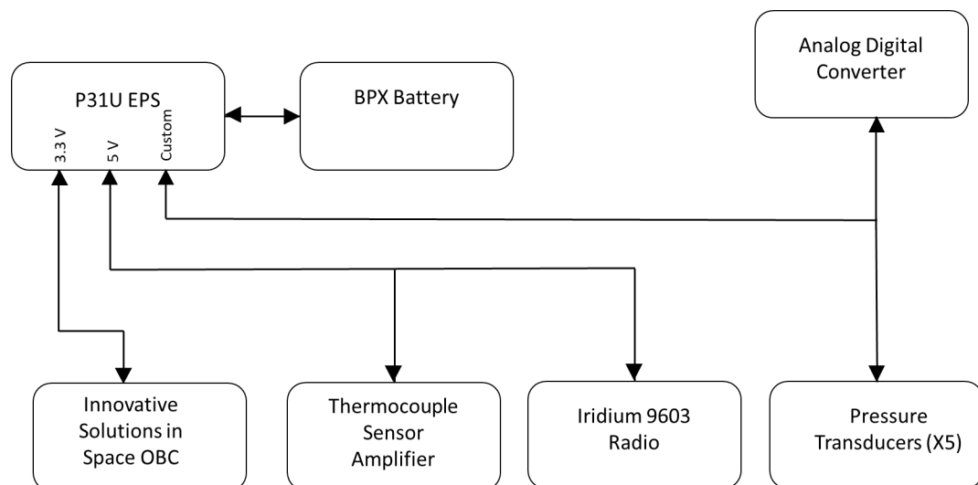
Figure 4. Power Flow Chart
