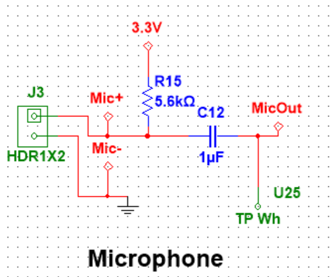
Figure 7: Microphone Circuit
