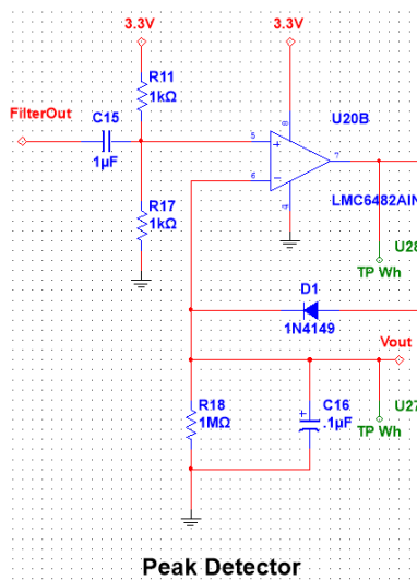
Figure 6: Peak Detector
