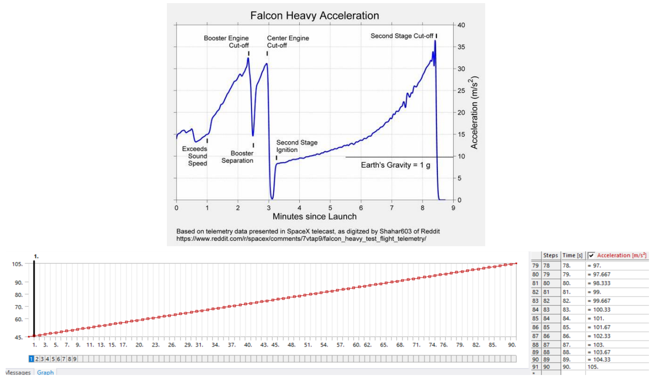
Figure 34: Falcon Heavy Acceleration
