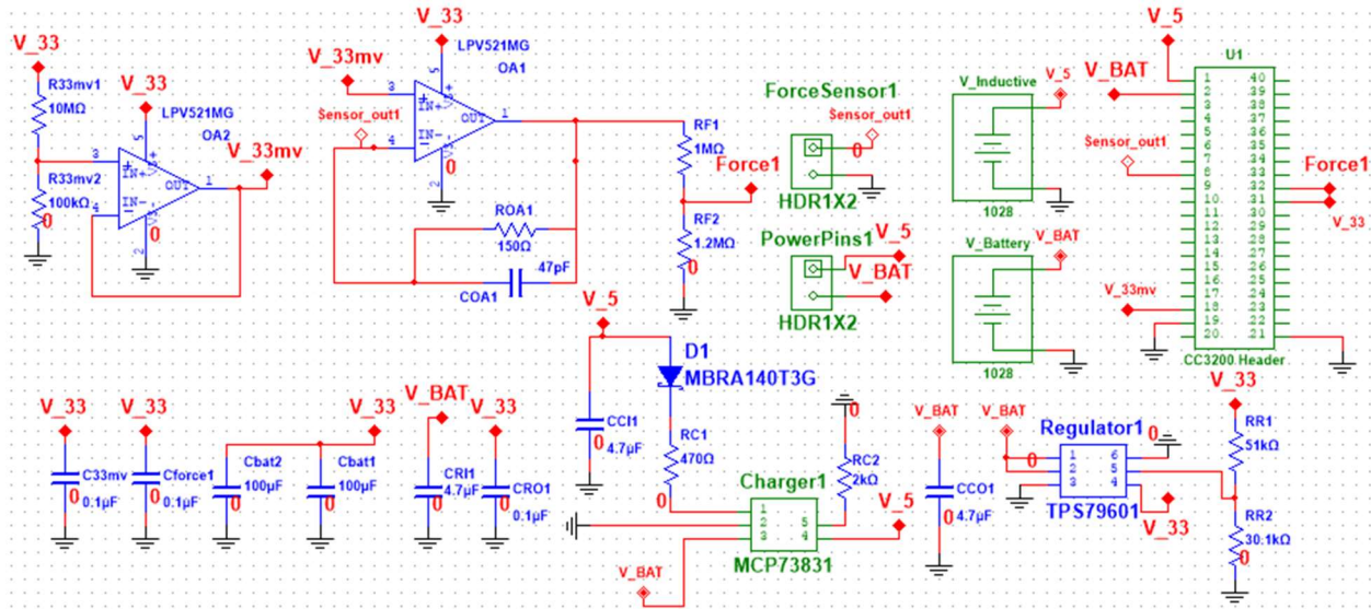
Figure 5 Header Schematic
