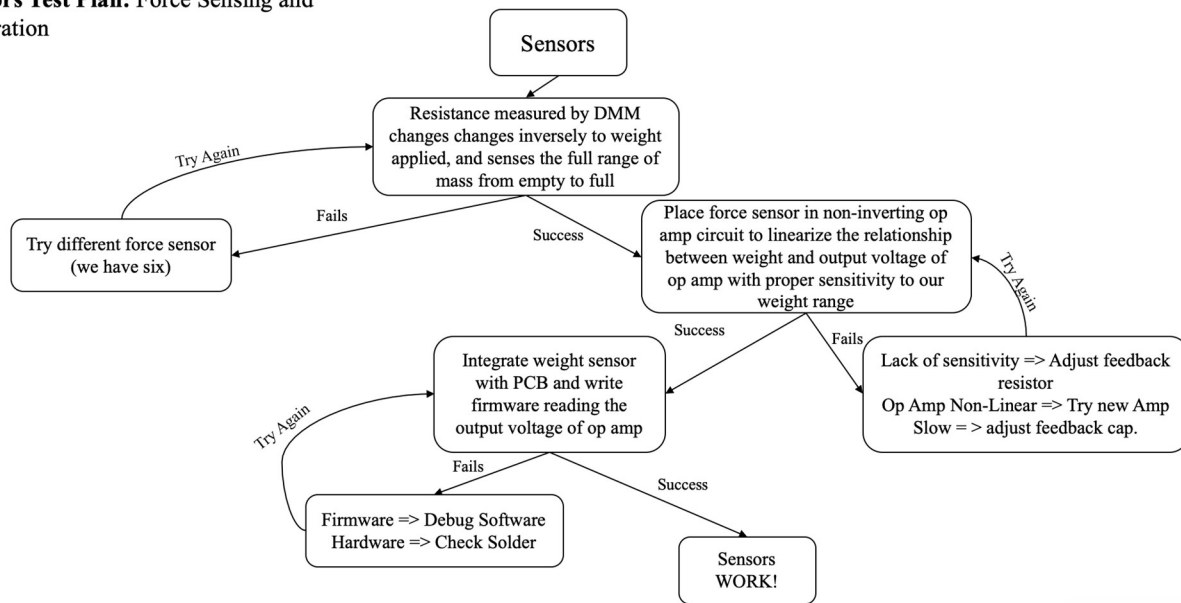
Figure 17 Sensors Test Plan
