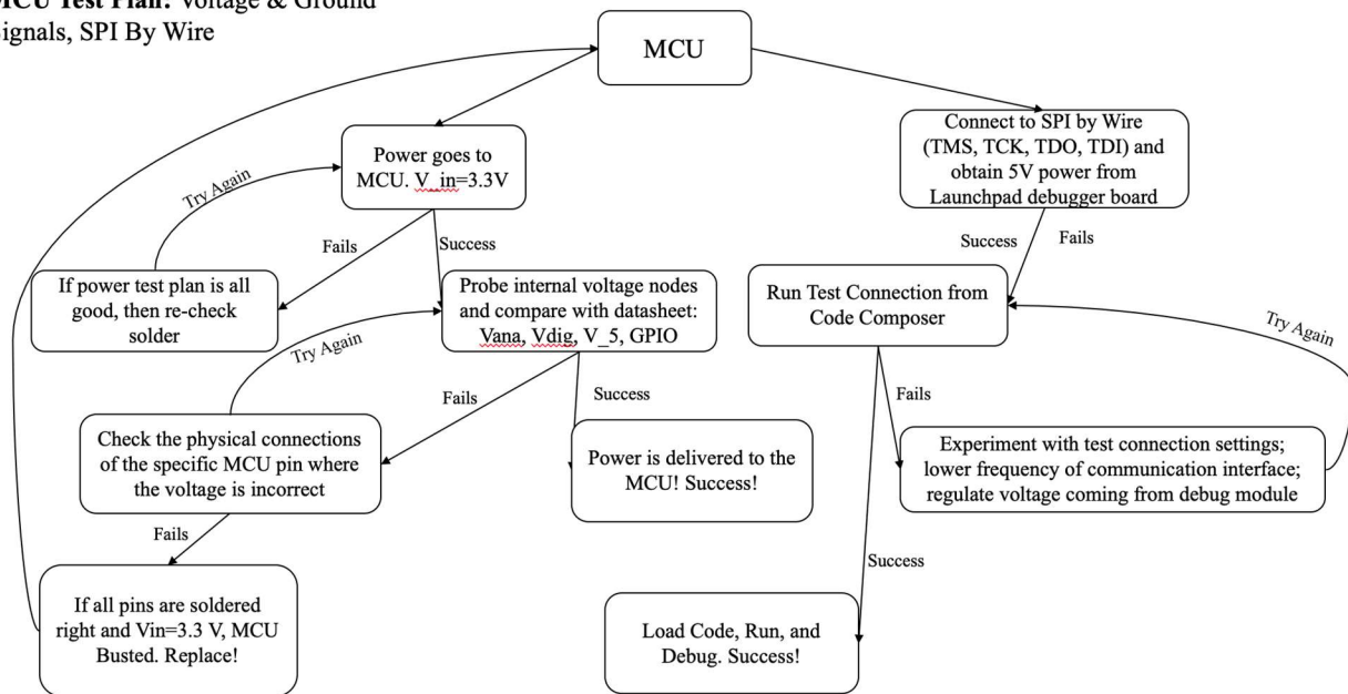
Figure 16 MCU Test Plan
