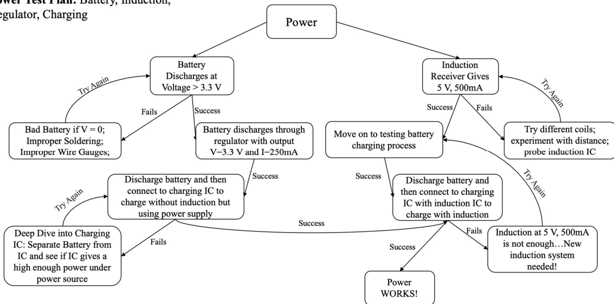
Figure 15 Power Test Plan
