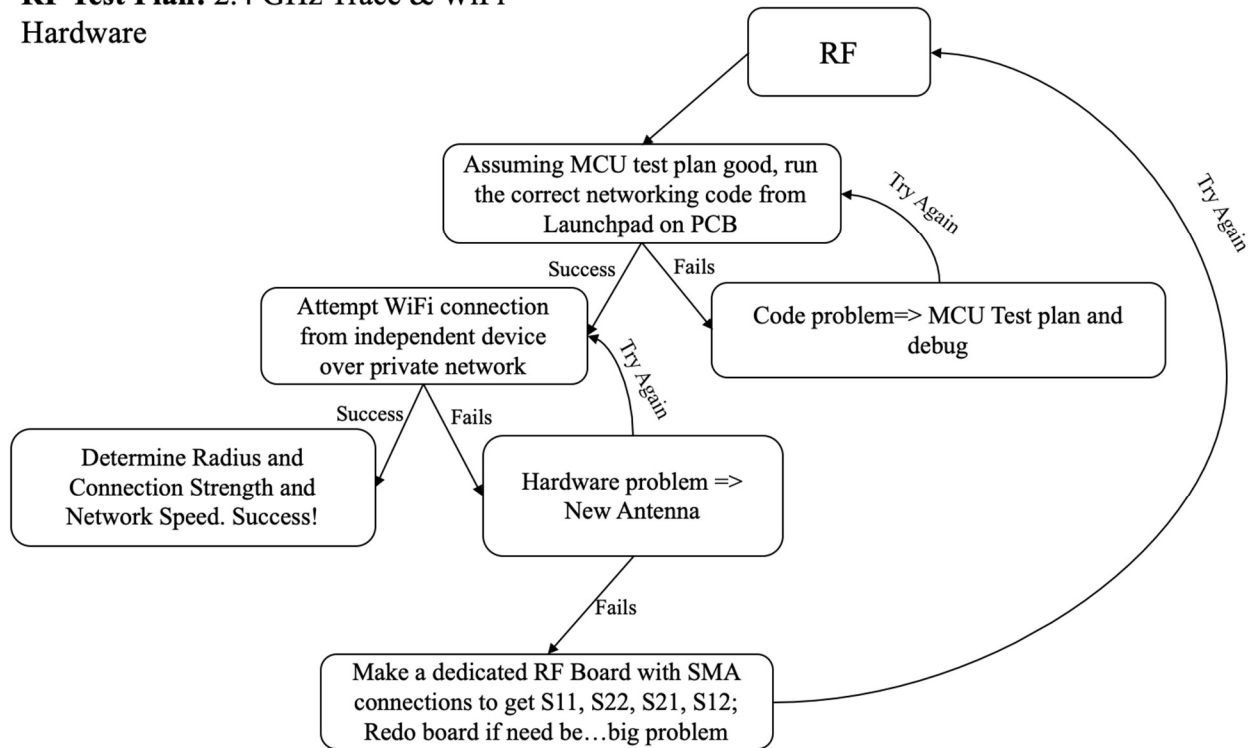
Figure 18 RF Test Plan
