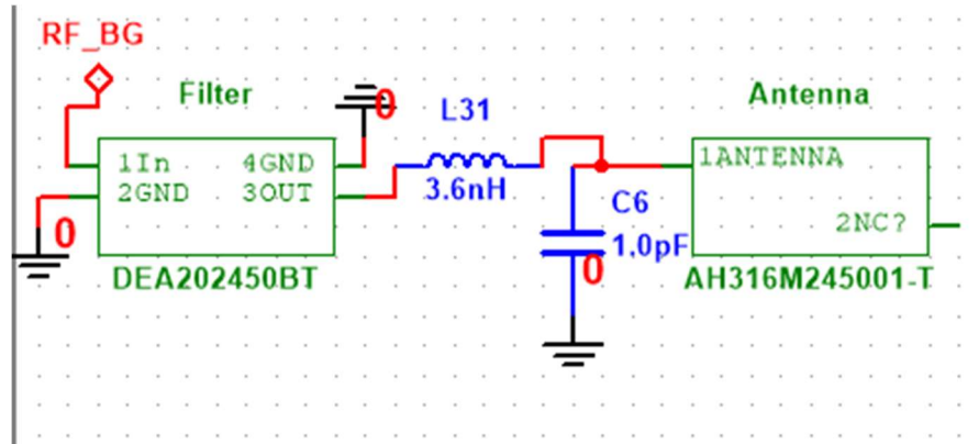
Figure 1 RF Schematic
