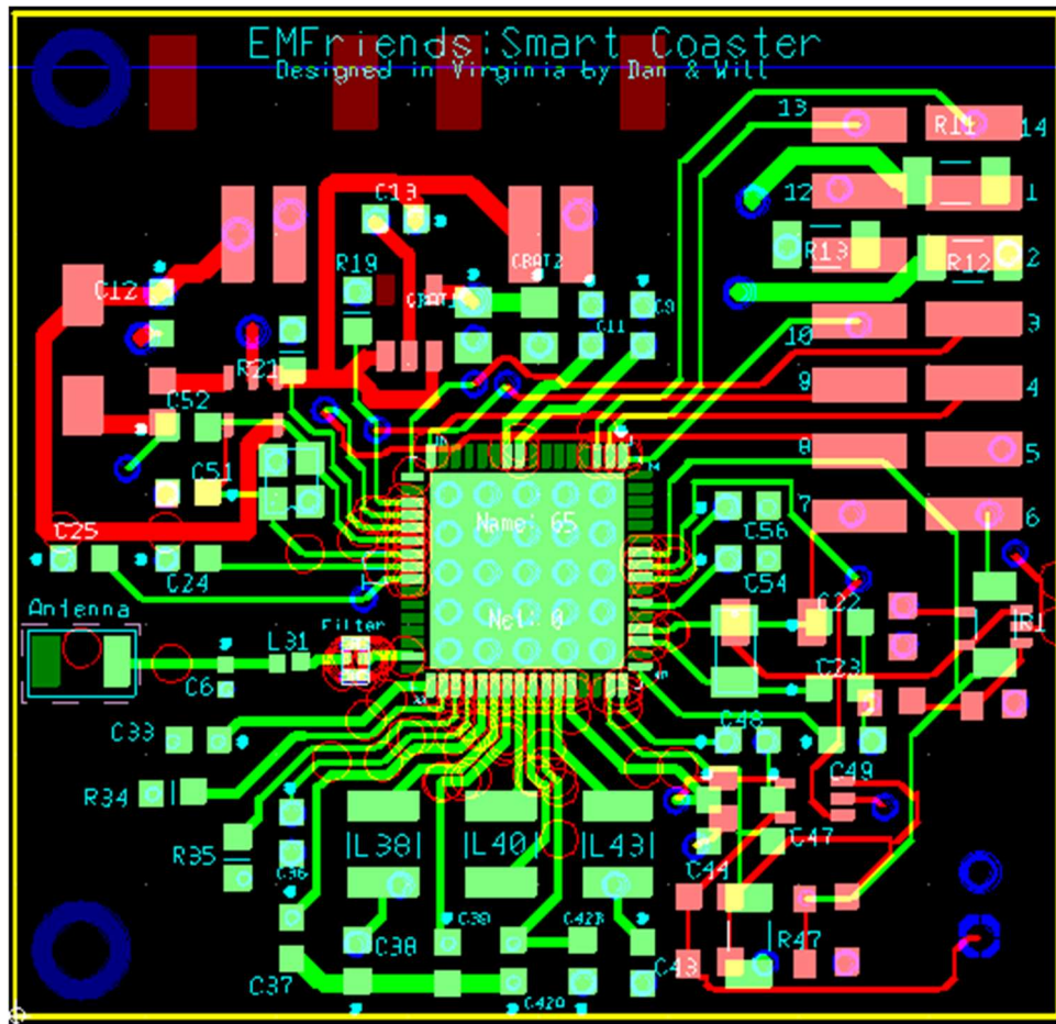
Figure 6 First Board Layout
