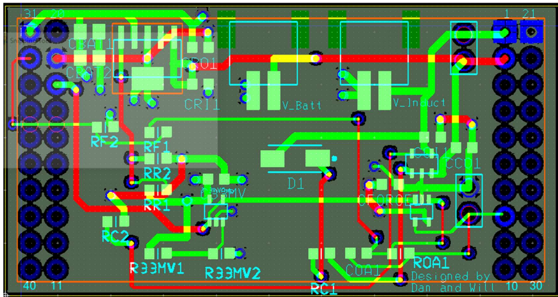
Figure 8 Header Board Layout
