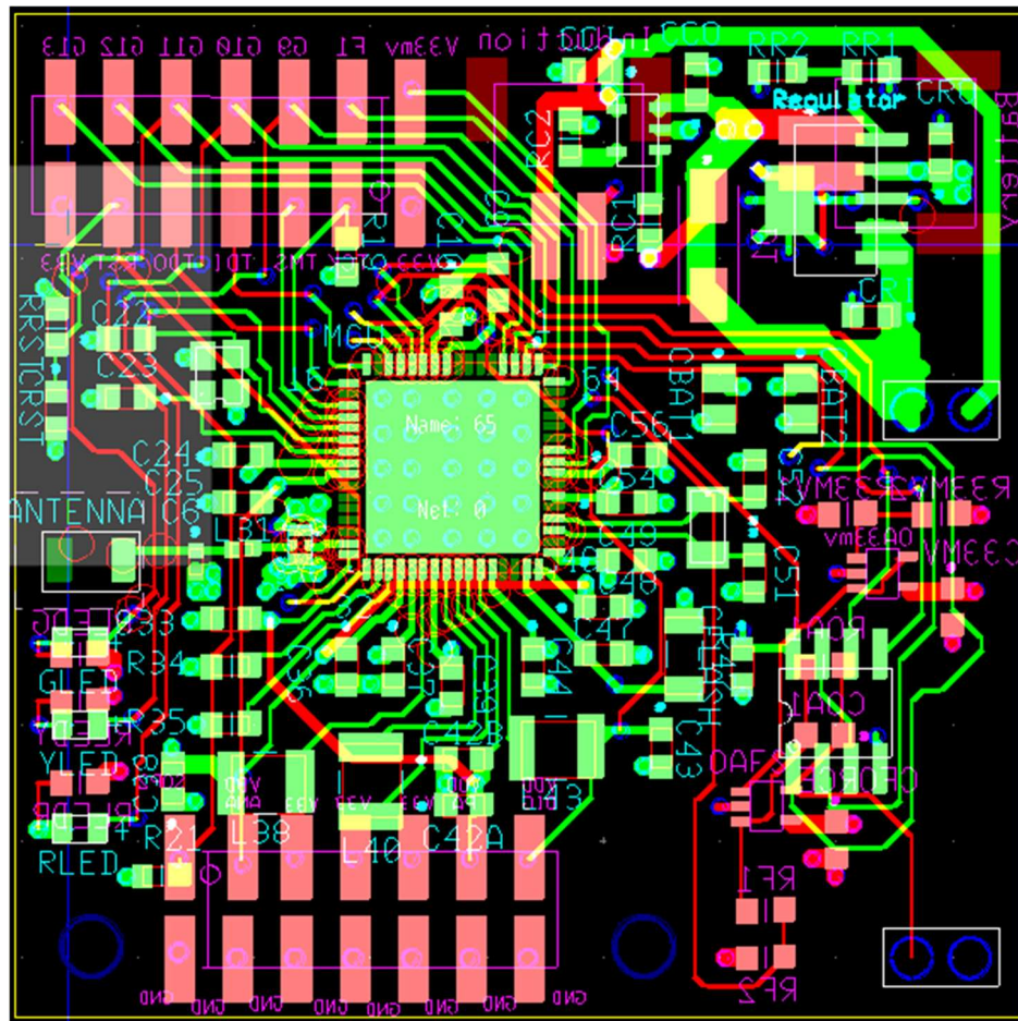
Figure 7 Second Board Layout
