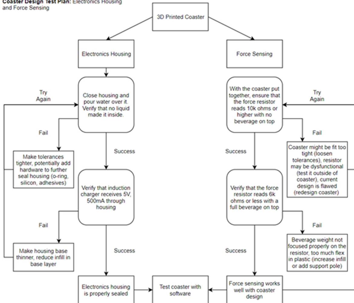
Figure 19 Coaster Design Test Plan
