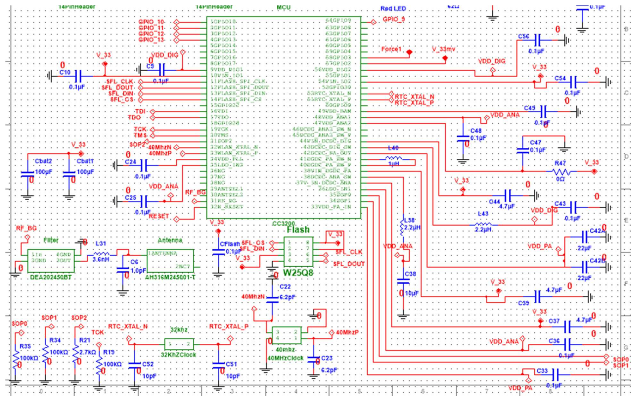
Figure 4 MCU Schematic
