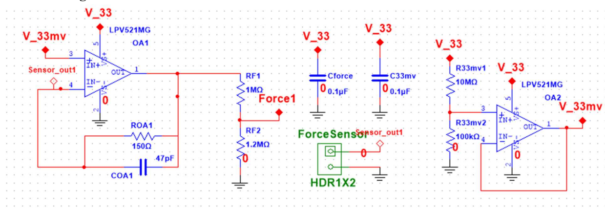
Figure 2 Force Sensing Schematic
