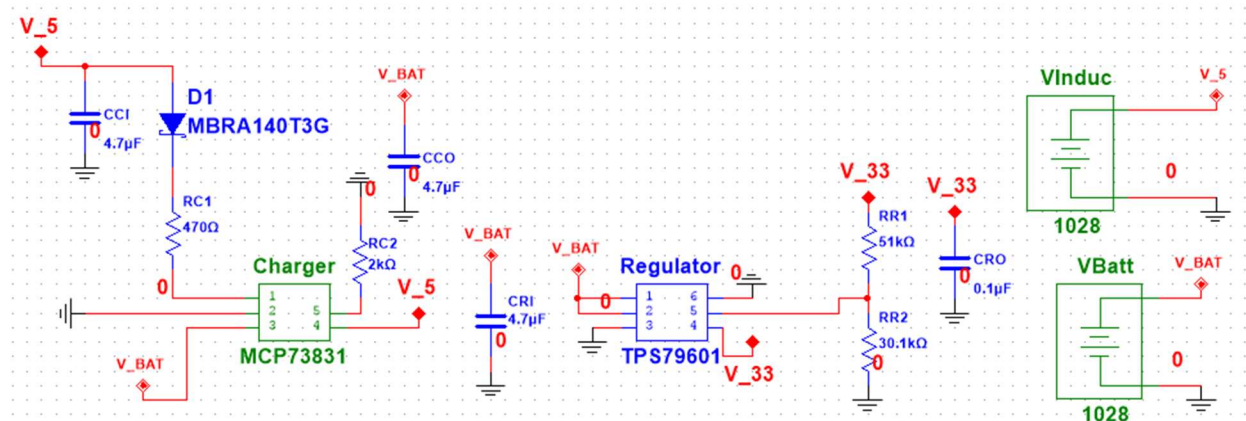
Figure 3 Power Schematic
