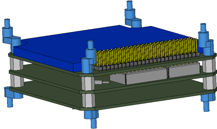
Figure 3: AMSAT Linear Transponder Module Stack With Custom Threaded Brackets
