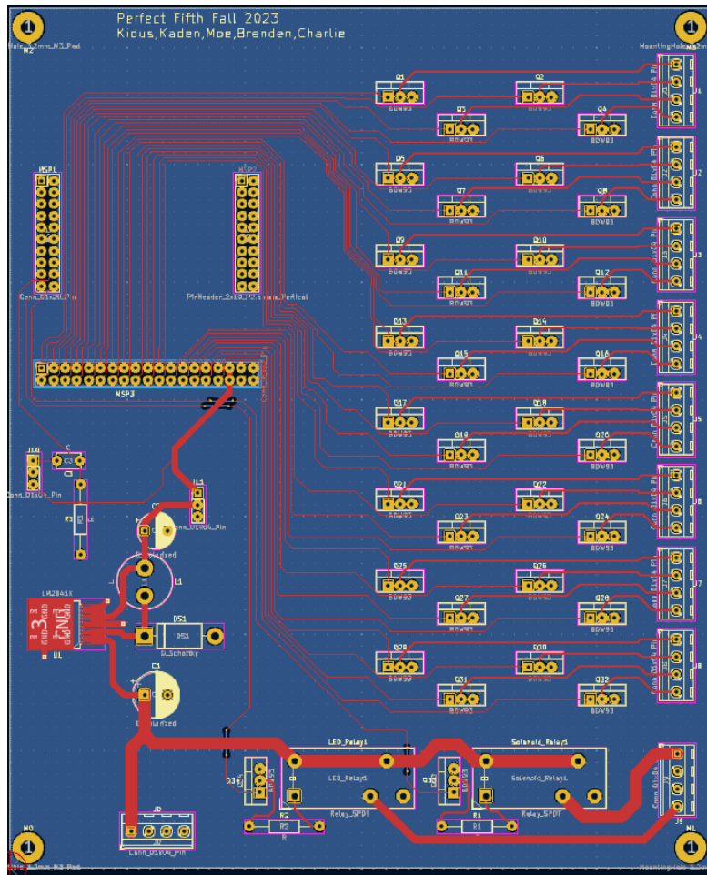
Figure 12 PCB Layout
