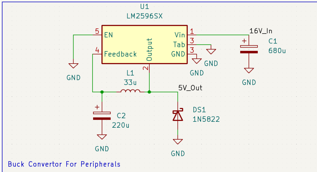
Figure 5 Buck Convertor Schematic
