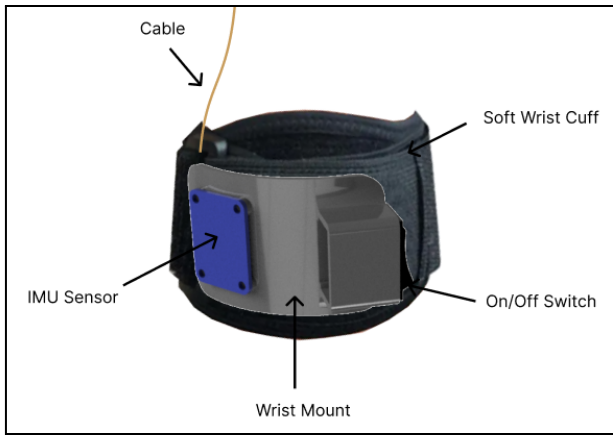
Fig 26. Wrist assembly
