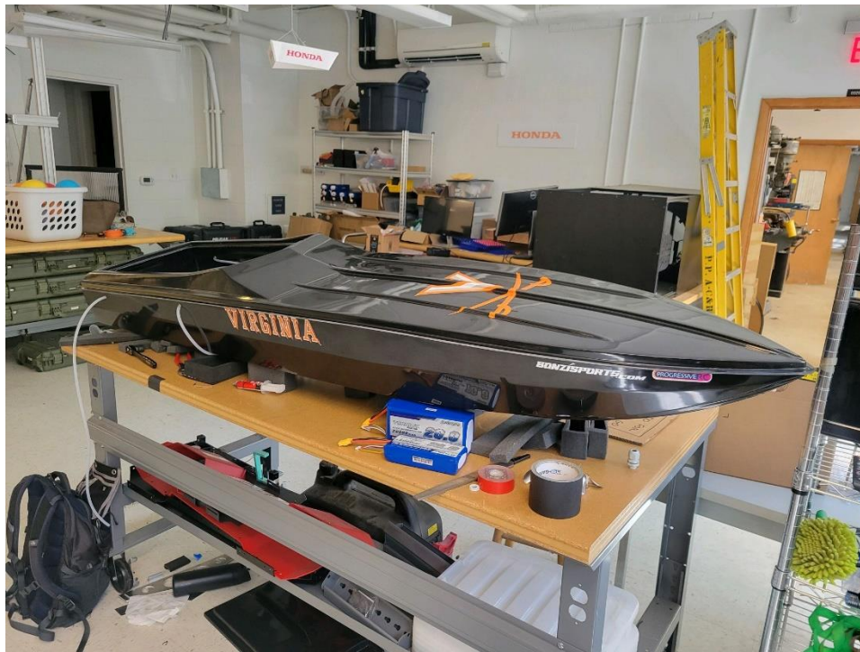
Figure 19: Outside View of Hull
