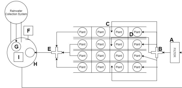
Fig. 2. Top View of Hydroponic System
