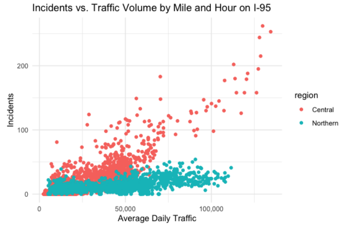
Fig. 3. Scatterplot of incidents vs. traffic volume controlling for region.
