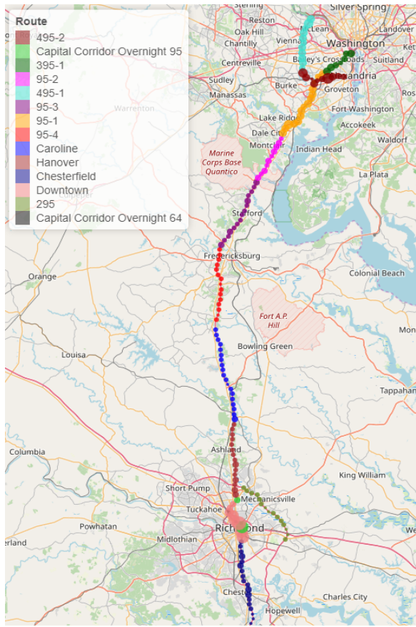
Fig. 1. Map of I-95 in Virginia with markers sized by incident density.
