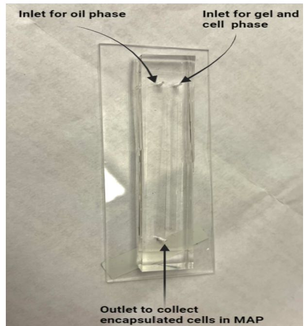
Figure 3: This is a picture of the microfluidic device that is utilized in the encapsulation runs. The inlet on the left is where the oil/surfactant solution goes. The inlet on the right is for the gel and cell solution. The outlet on the bottom is to collect the final solution.
