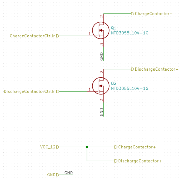
Figure 11. Contactor Control Schematic
