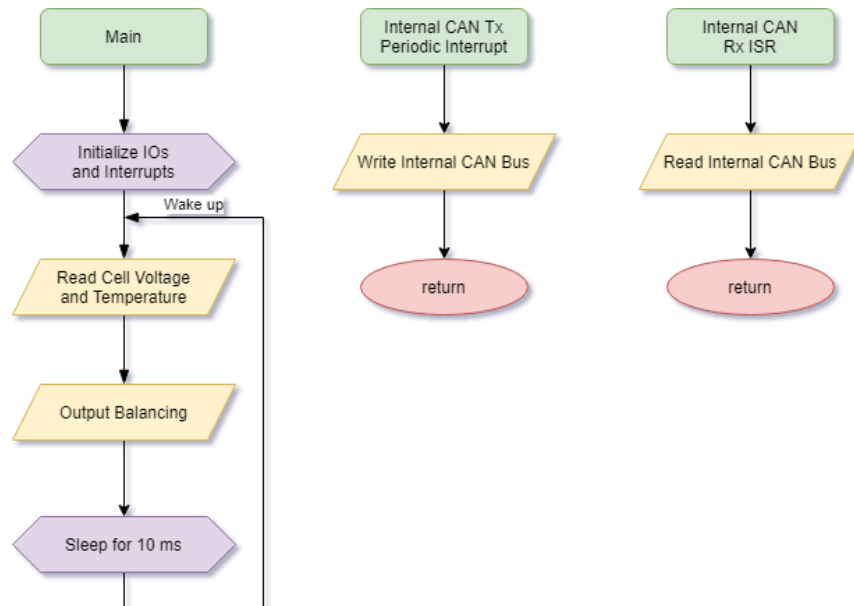
Figure 23. Cell Node Software Flow Chart
