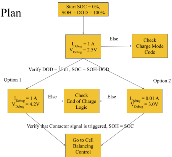
Figure 44. SOC Discharging Test Plan
