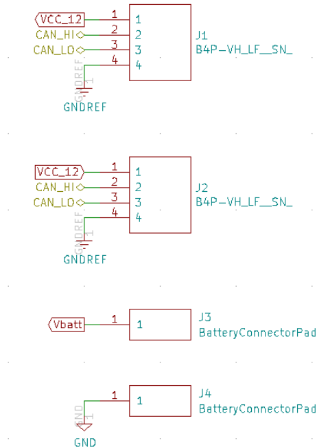
Figure 17. Cell Node Connectors Schematics
