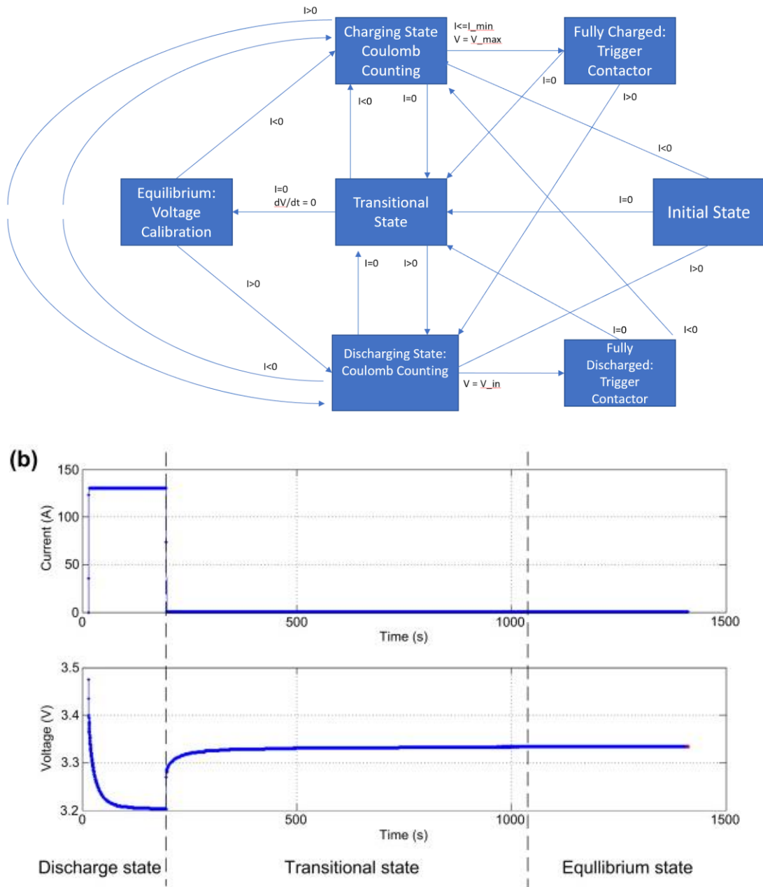
Figure 29. State Diagram of Combined Coulomb Counting and Voltage-based for SOC Estimation
