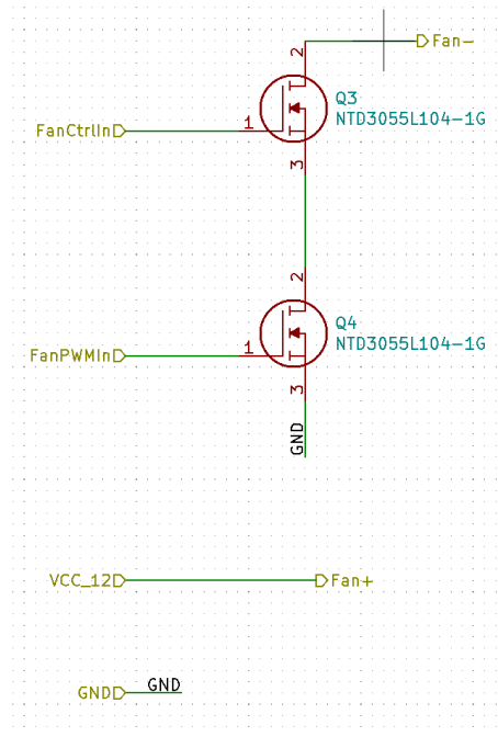
Figure 10. Fan Control Schematic
