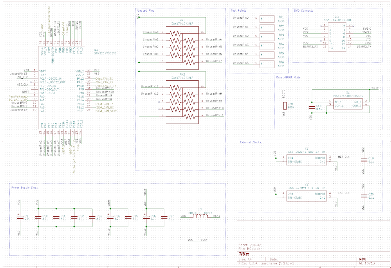
Figure 4. Main Node MCU Schematic
