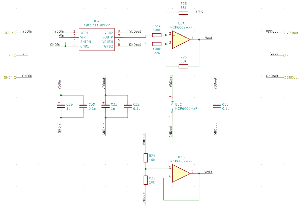
Figure 9. Isolation Schematic
