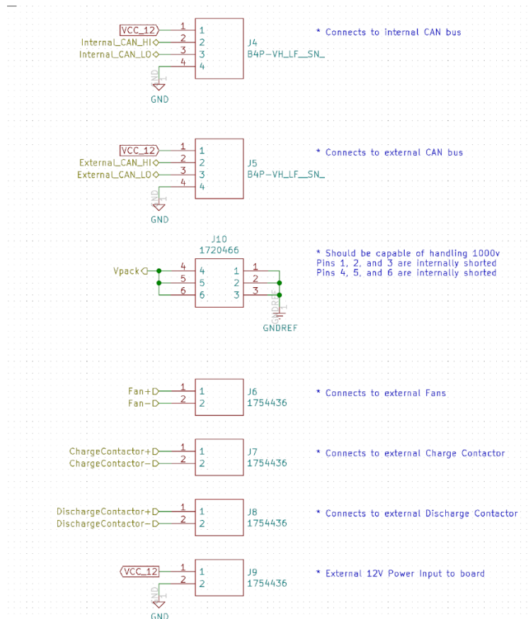
Figure 5. Connectors Schematic
