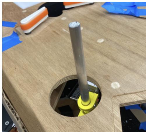
Fig. 2.3.4. First iteration of pop bumper mounted to playfield (top view)
