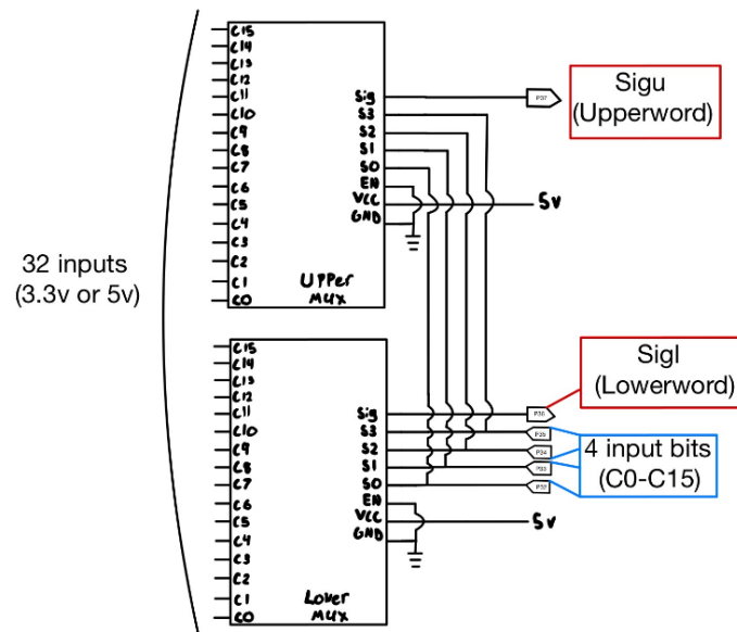
Fig. 4.3.1. Wiring diagram for two parallel multiplexers
