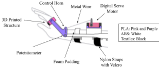
Figure 10: Wrist Exoskeleton Components and Materials
