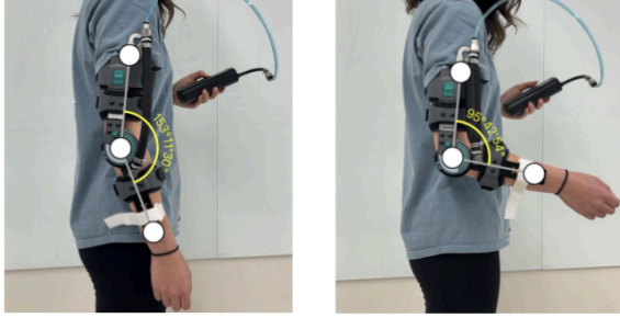
Figure 13: First Prototype of Elbow Design
