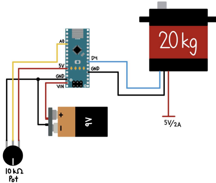
Figure 11: Basic Circuit Layout for Wrist Components
