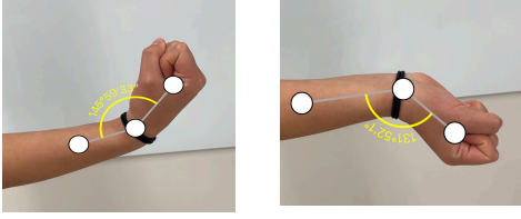
Figure 3: Natural Human Wrist Flexion and Extension
