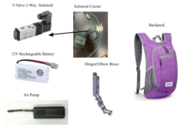
Figure 8: Backpack and Components
