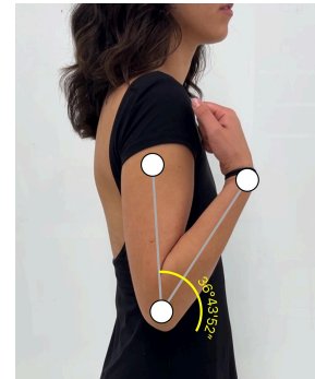
Figure 2: Natural Human Elbow Movement Due to Bicep Contraction
