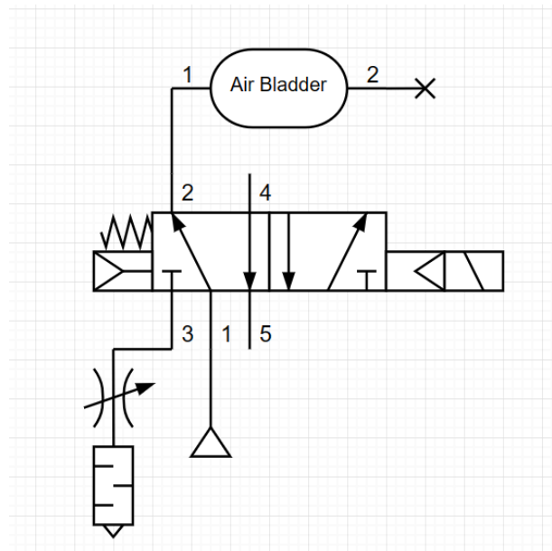
Figure 9: Schematic of Solenoid Pneumatic Design
