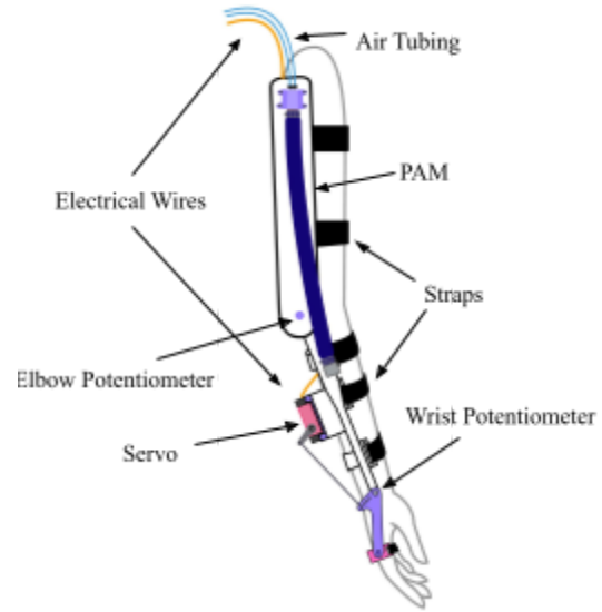
Figure 1: Overview of the W.E.A.R. Bot Exoskeleton (Backpack Containing Air Pump, Solenoid, Arduino, and Power Supply Not Pictured)
