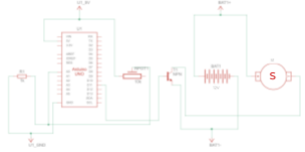
Figure 6: Circuit for Solenoid and Potentiometer
