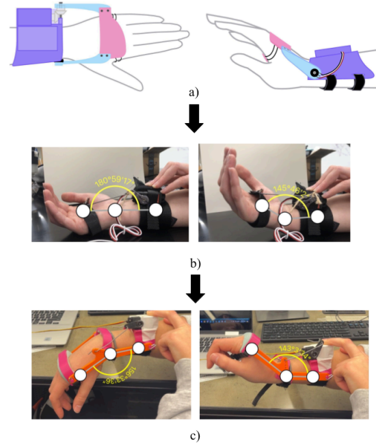
Figure 15: Wrist mechanism design iterations, a) initial design sketch, b) first prototype, c) second prototype
