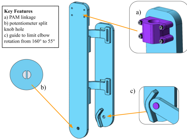
Figure 14: CAD of upper arm/bicep components of our final W.E.A.R. Bot brace, highlighting key features related to the elbow mechanism
