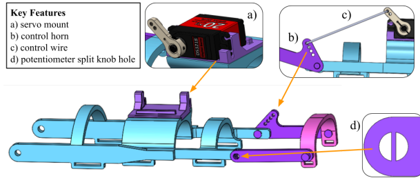
Figure 16: CAD of forearm and hand components in our final W.E.A.R. Bot brace, highlighting key features related to the wrist mechanism
