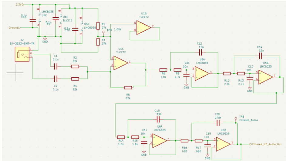
Figure 8: Audio Input Circuit Schematic
