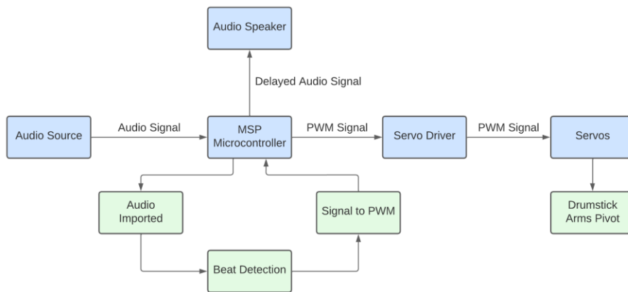
Figure 2: Whiplash Block Diagram
