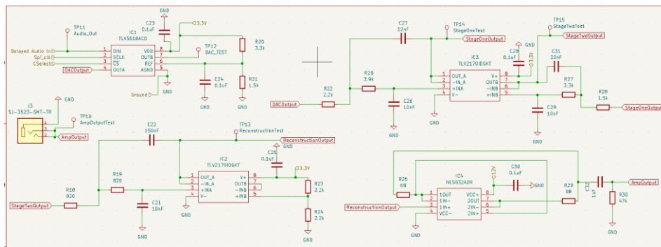
Figure 9: Audio Output Circuit Schematic
