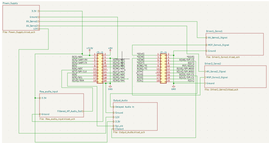
Figure 4: Top Level Schematic
