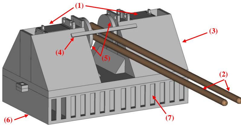
Figure 3: Whiplash 3D Model
