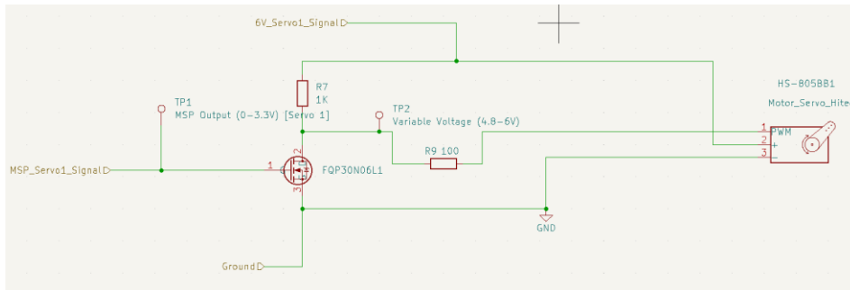
Figure 6: Servo Driver 1 Circuit Schematic
