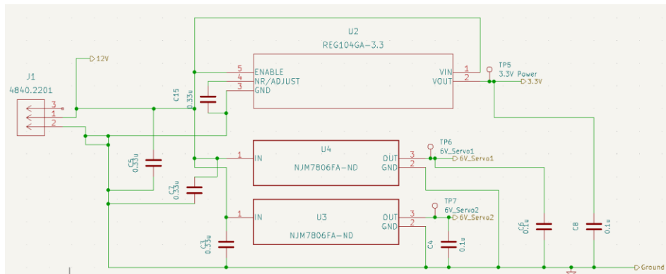
Figure 5: Power Supply Circuit Schematic
