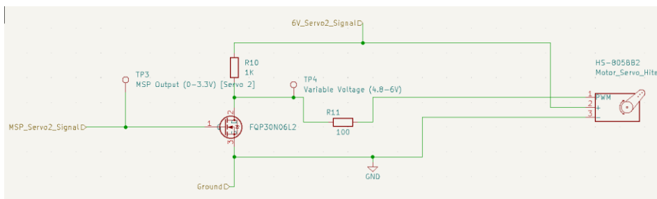
Figure 7: Servo Driver 2 Circuit Schematic
