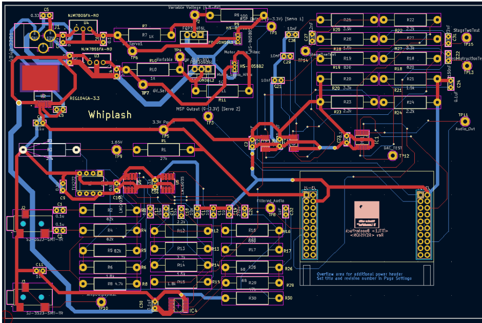
Figure 10: PCB Schematic
