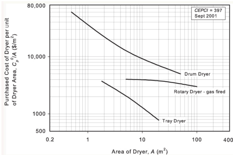
Figure B.1: Purchased Costs For Dryers (Turton, 2012)
