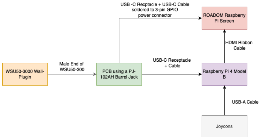
Figure 2: Block Diagram of the Hardware Connections
