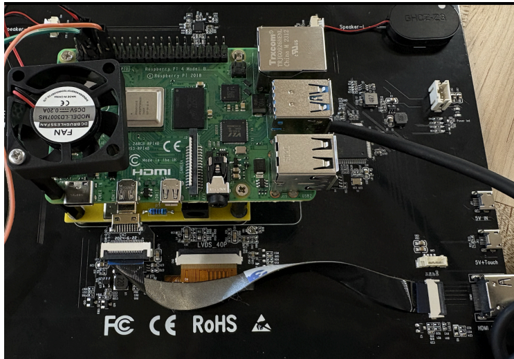
Figure 3: HDMI Ribbon Connection to the Screen.
