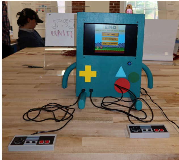
Figure 16: Completed EMO with Screen, Power Button, and Joystick Controllers Connected
