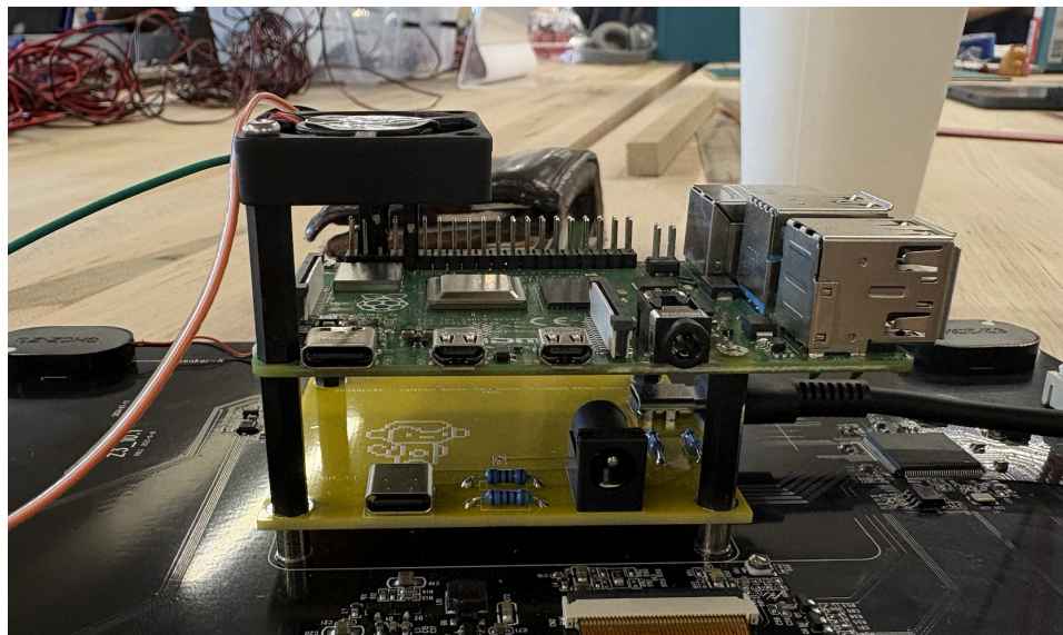
Figure 10: Stacked PCB and Raspberry Pi
