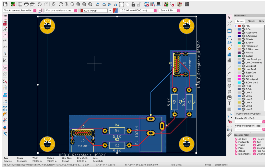
Figure 7: PCB Layout
