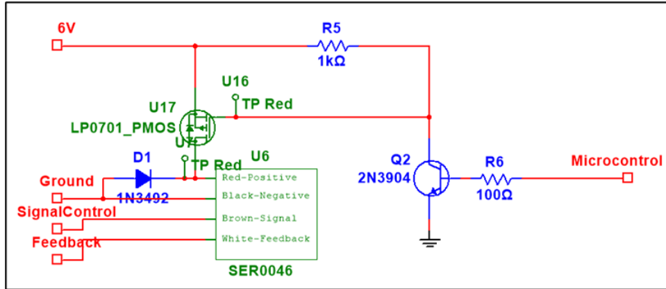
Figure 8: Servomotor Sub-Schematic
