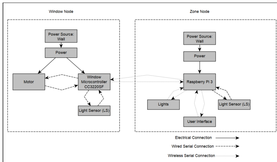
Figure 4: System Diagram
