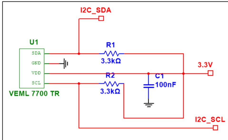
Figure 7: Light Sensor Sub-Schematic
