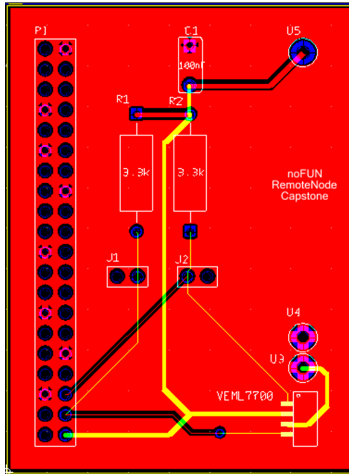
Figure 11: Remote Node Ultiboard Design
