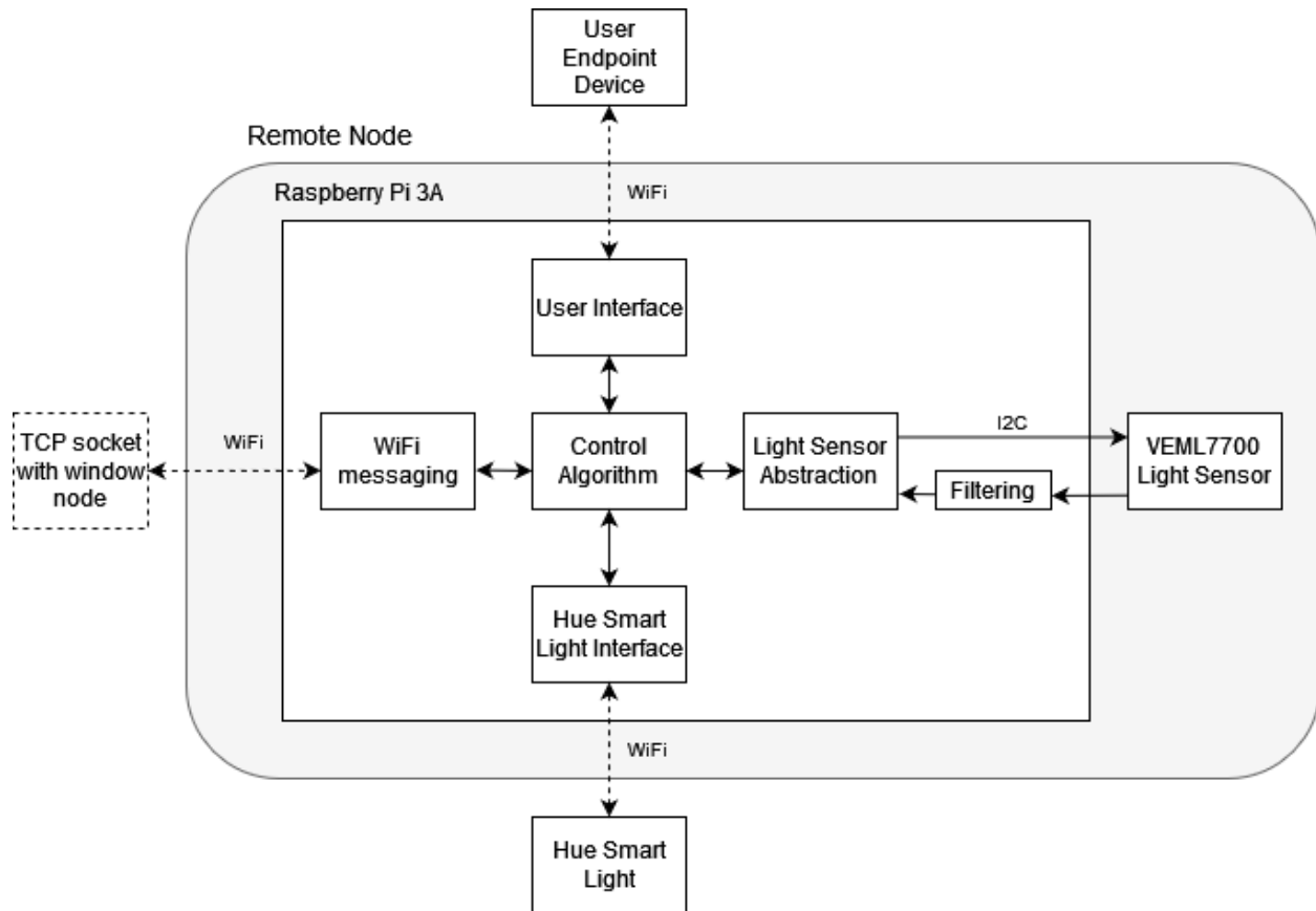
Figure 14: Data Flow Diagram for Remote Node
