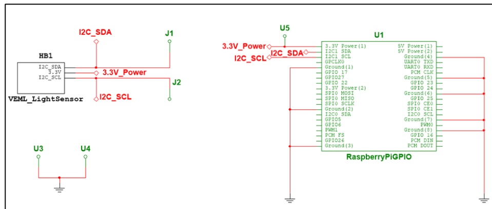
Figure 10: Remote Node Schematic
