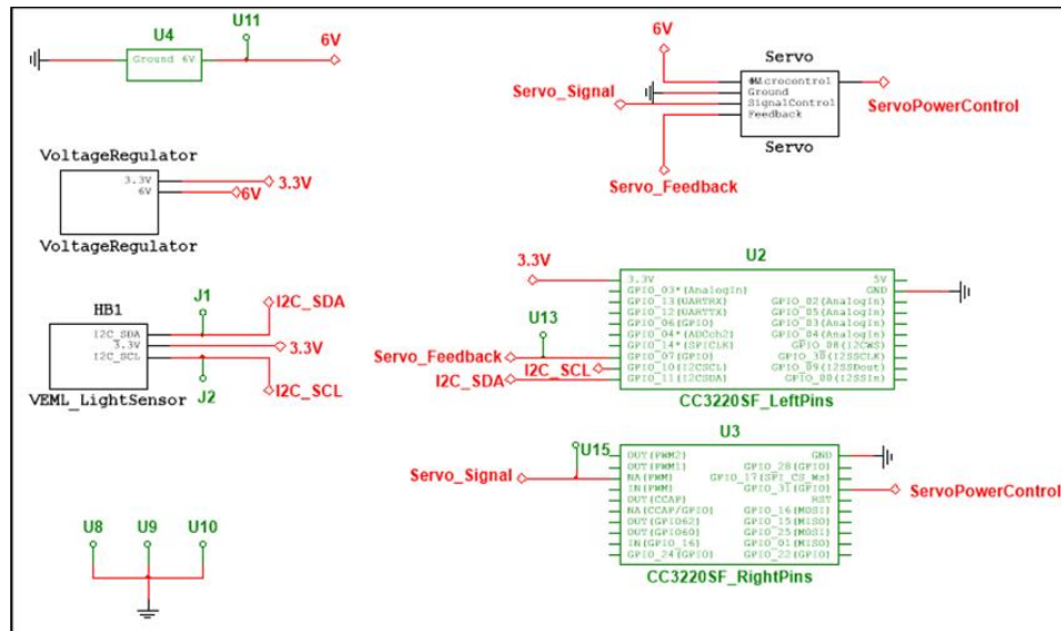
Figure 5: Window Node Schematic
