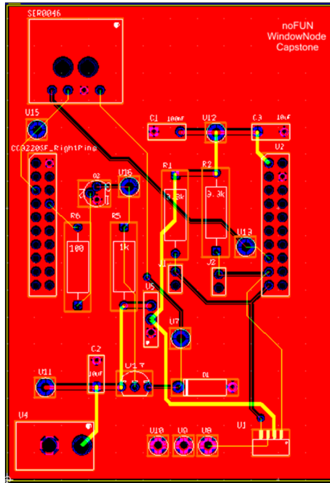
Figure 9: Window Node Ultiboard Design
