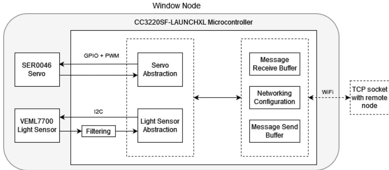
Figure 12: Data Flow Diagram for Window Node
