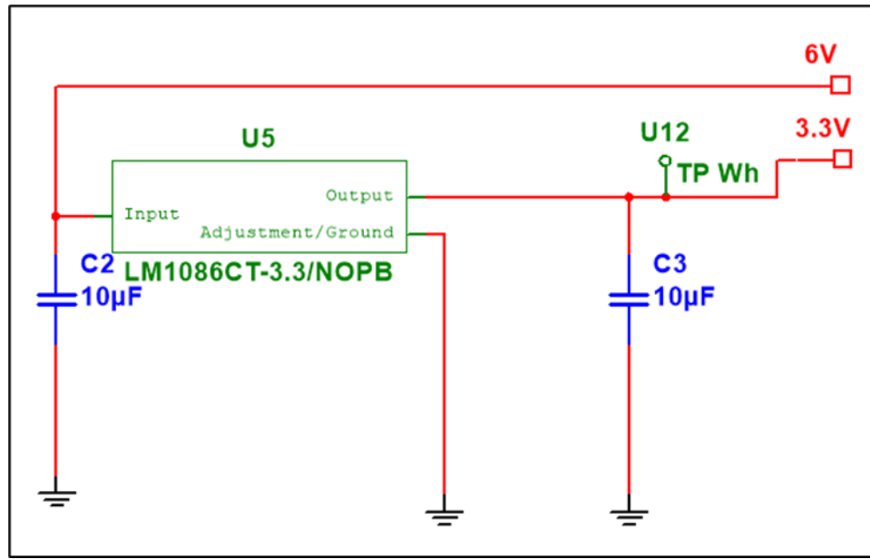
Figure 6: Voltage Regulator Schematic
