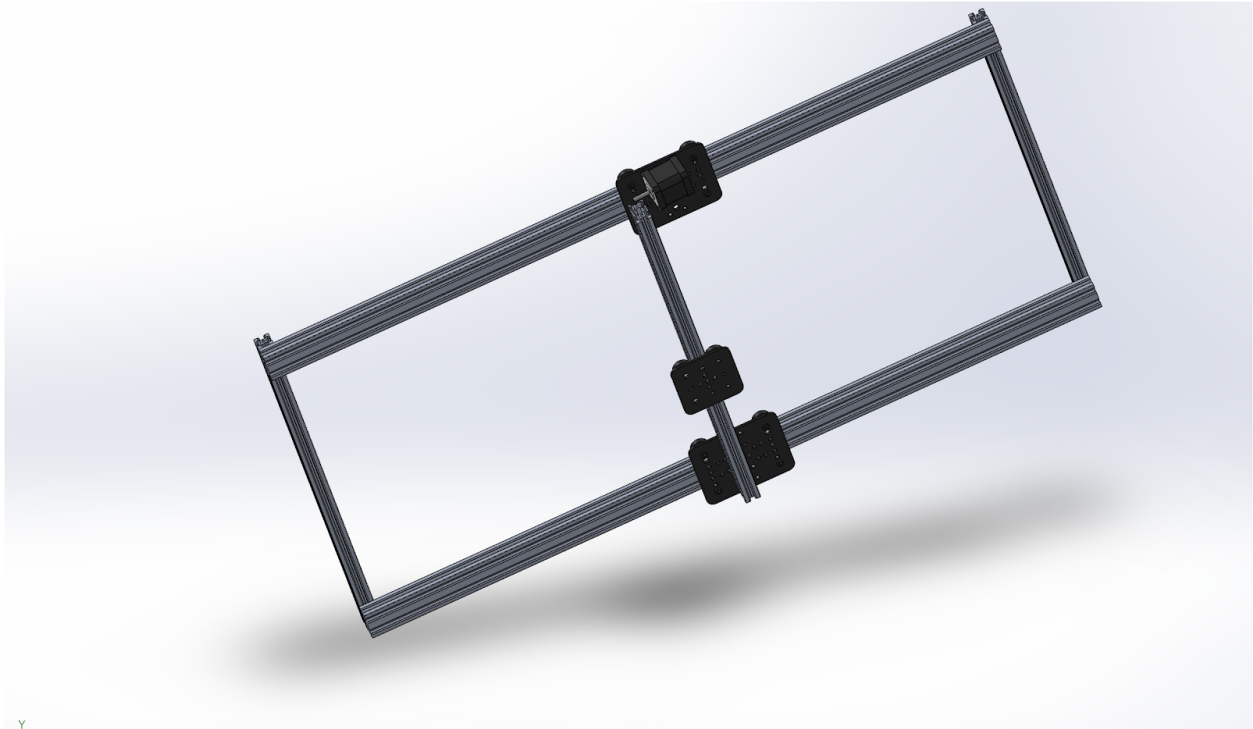
Figure 10: CAD rendering of frame, carts, and crossbar
