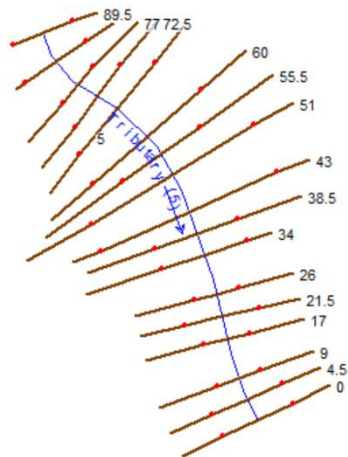
Reach 5 HEC-RAS Model Layout with Cross Sections at Delineated Stations
