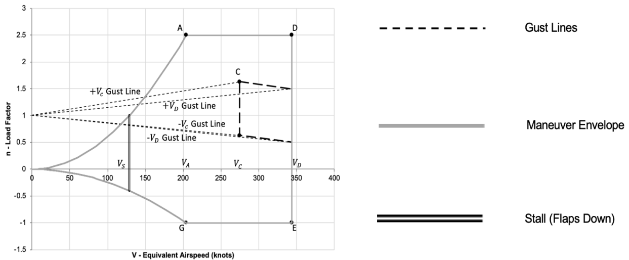
Figure XI-1. V-N Diagram
