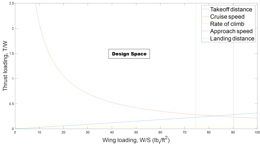
Figure IV-1. Constraint Diagram
