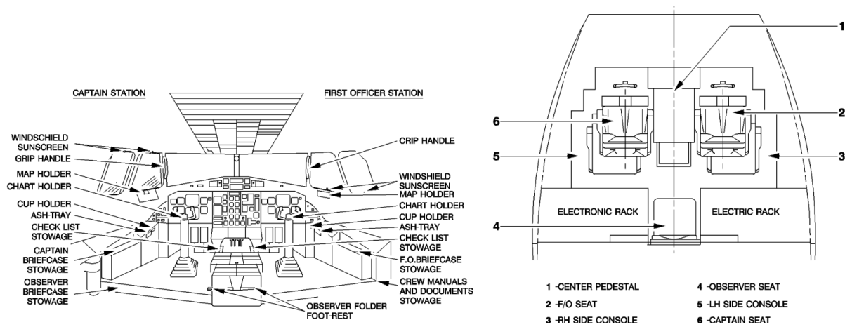
Figure V-3. Cockpit Diagram
