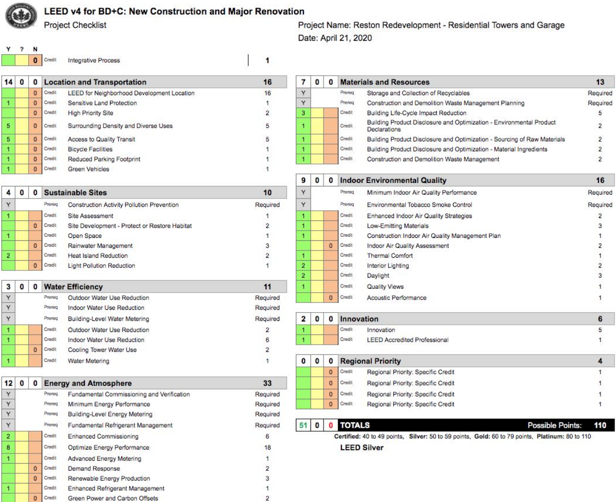
Figure 1: LEED Scorecard - Residential Buildings
