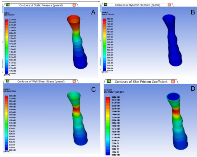
Figure 4. Modeling Results from CFD analysis of Patient 3. A) Contour of Static Pressure B) Contour of Dynamic Pressure C) Contours of Wall Shear Stress. D) Contour of Skin Friction Coefficient
