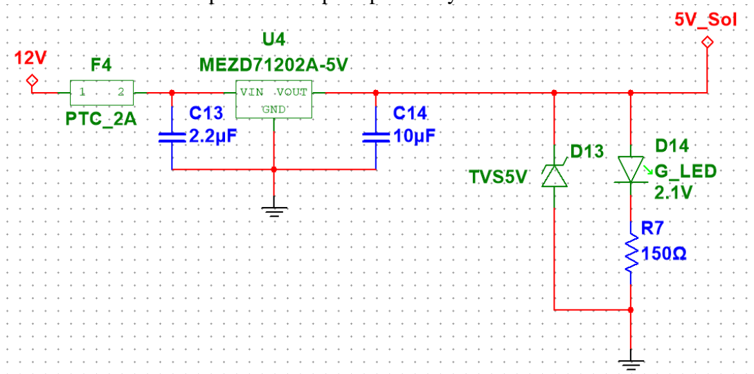
Figure 7 5V 2A DC to DC
