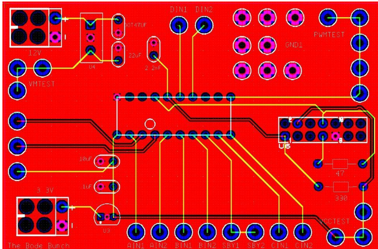
Figure 8 Ultiboard Schematic
