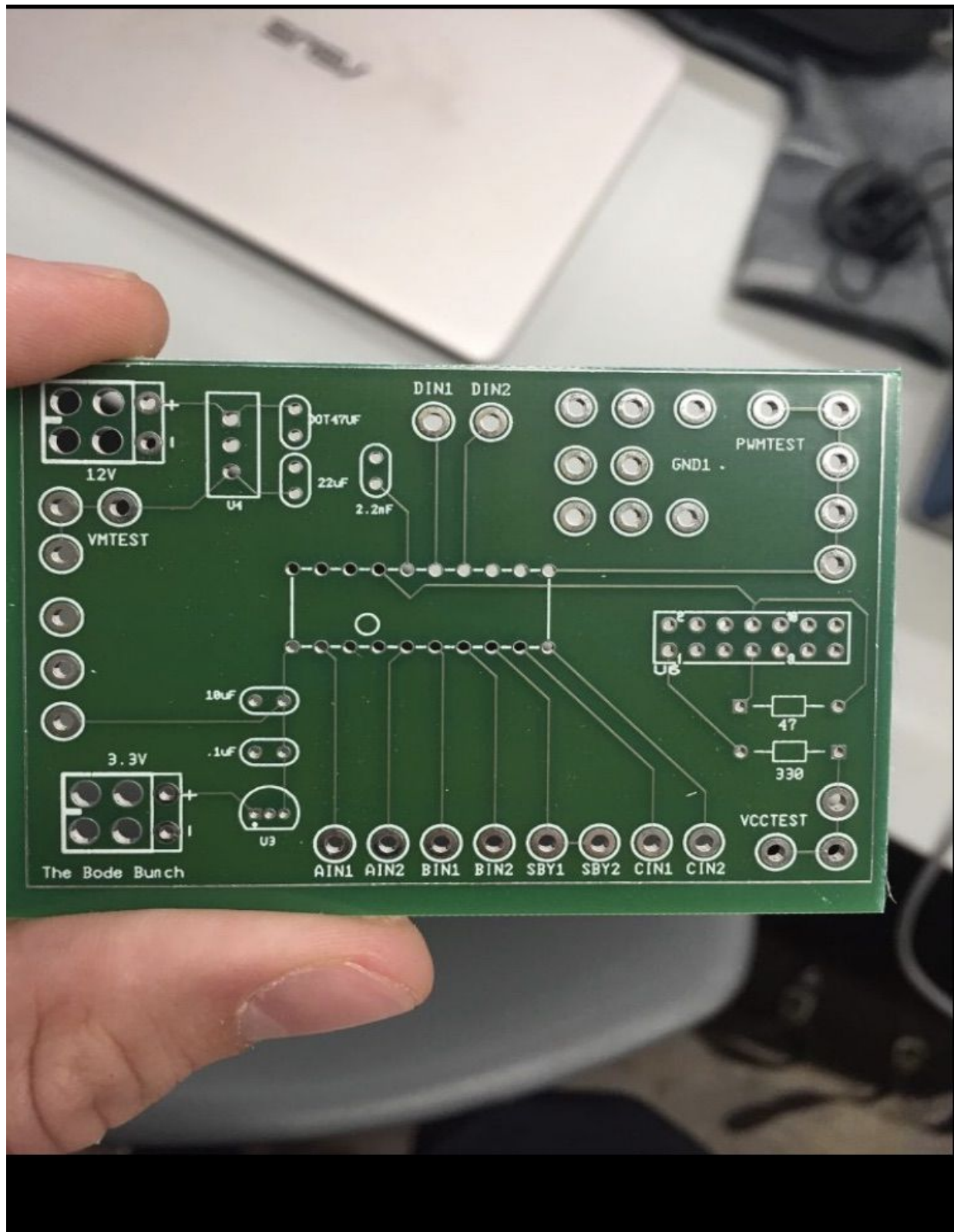
Figure 9 PCB Picture
