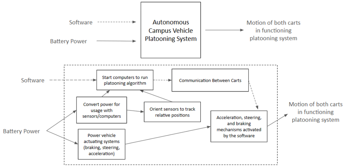
Fig. 3: Diagram of Functional Decomposition
