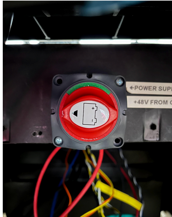
Fig. 22: Power switch
