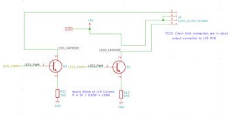
Figure 7. LED Driver Circuit Schematic
