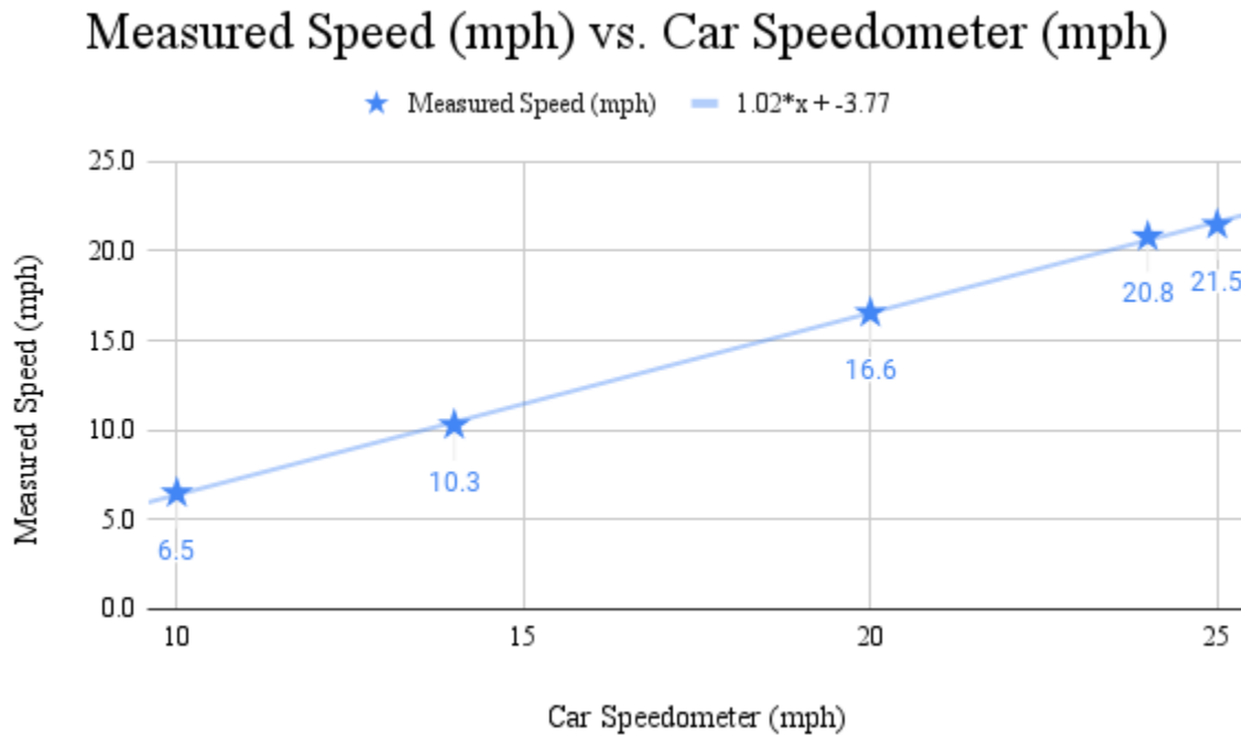
Figure 19. Measured Speed vs. Car Speedometer for Sensor Validation
