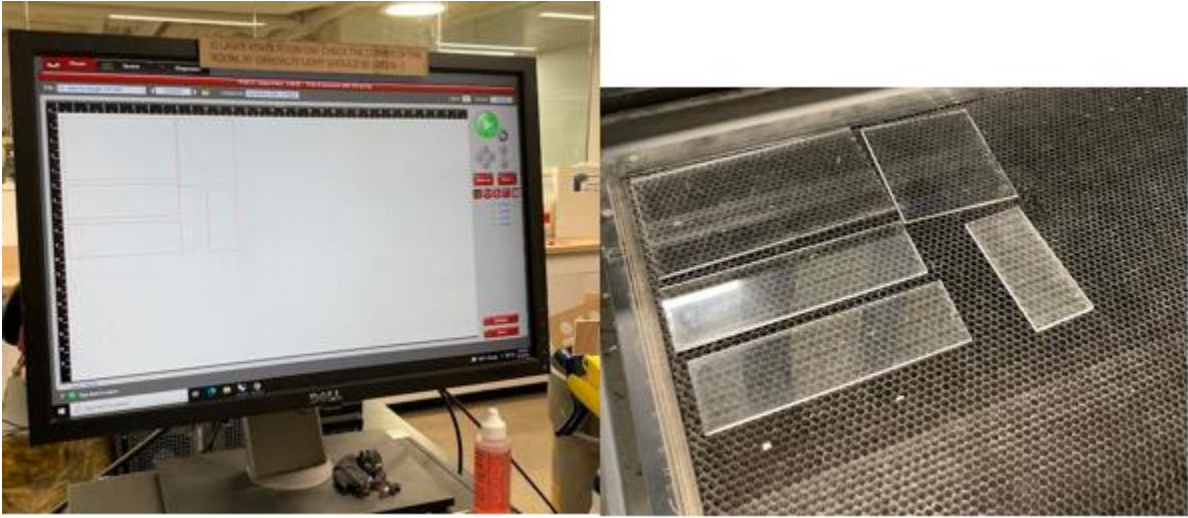
Figure 28. Laser Cutting Process
