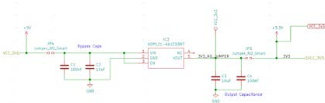
Figure 6. Linear Voltage Regulator Circuit
