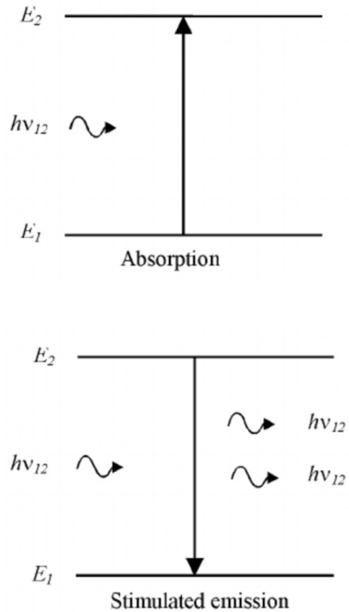
Figure 1. Laser Mechanism in Atomic Level (Kitching et al. [10])
