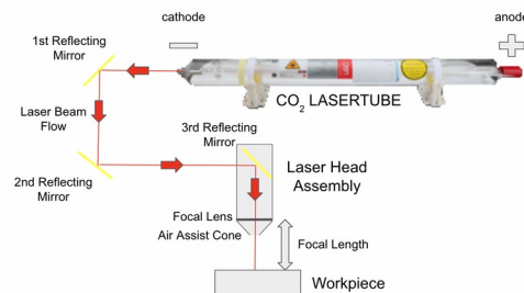
Figure 8 . Optical Layout Diagram
