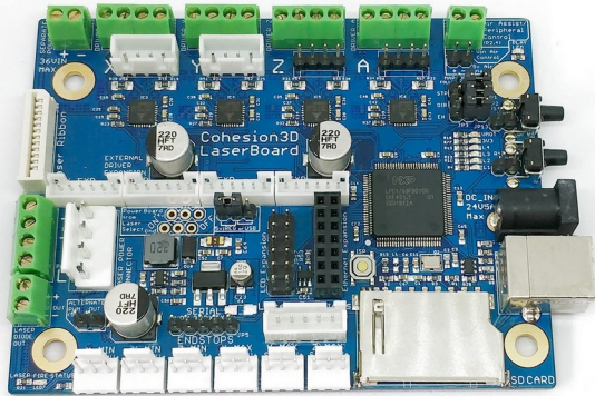
Figure 5. Cohesion 3D Laser Board (Cohesion3D [13])
