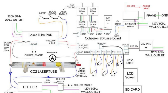
Figure 6 . Electrical Wiring Diagram
