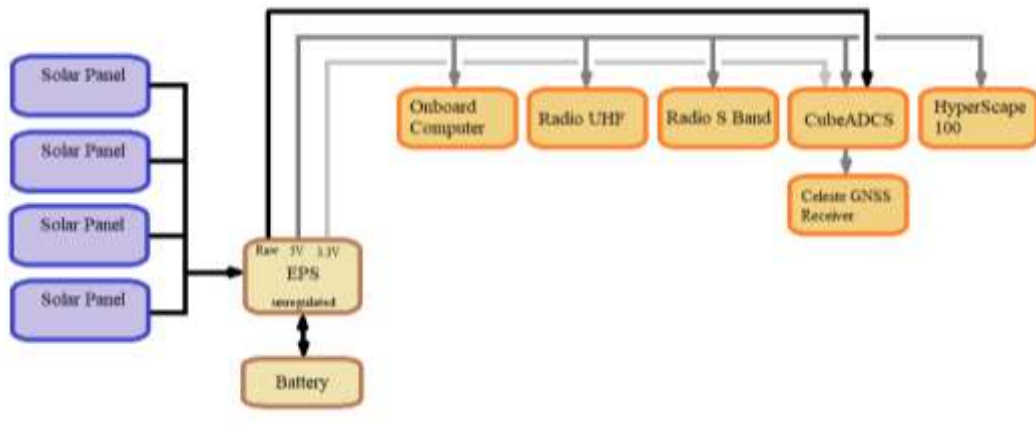
Figure 4. Power flow chart for CLAYTON. This figure depicts the generation, processing, and distribution of power for each component.
