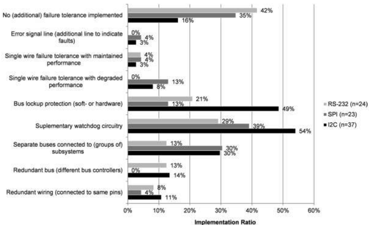
Figure 2. Implementation of failure tolerance features in CubeSats for different data buses based on “Survey on the implementation and reliability of CubeSat electrical bus interfaces”
