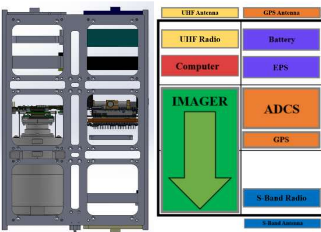
Figure 7. Diagram of each major component in the CubeSat and where it is located (right), CAD Model including all parts except solar panels (left)
