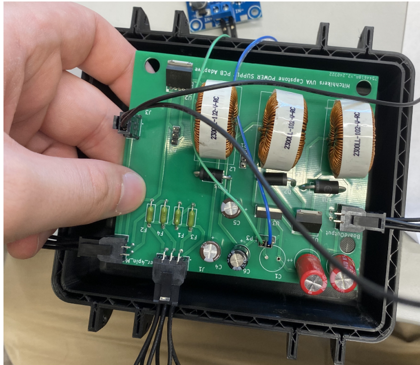
Figure 11: Power board in its 3D printed enclosure.
