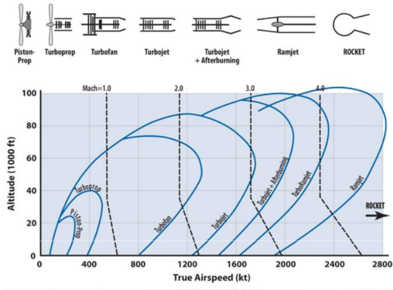
Figure 4.6 Level-flight propulsion options.
