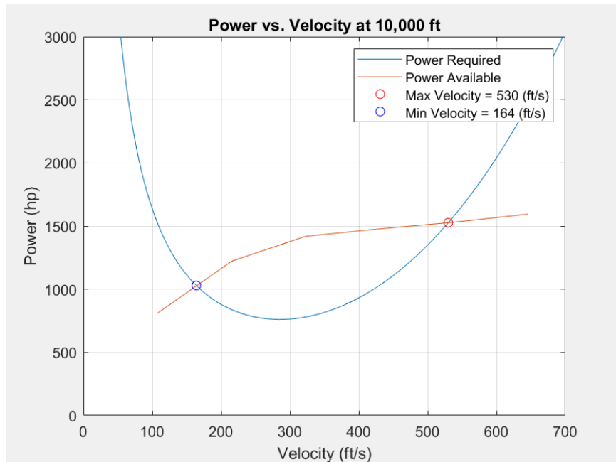
Figure 24: Power Curve
