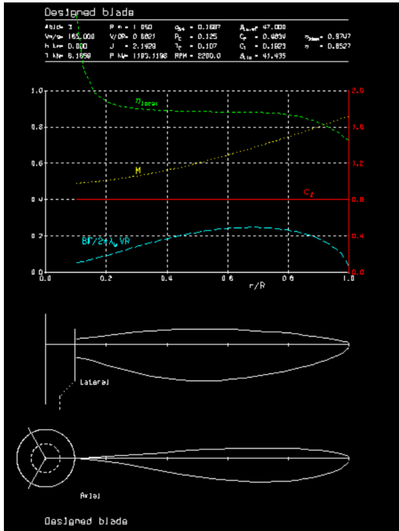
Figure 17: XROTOR propeller design
