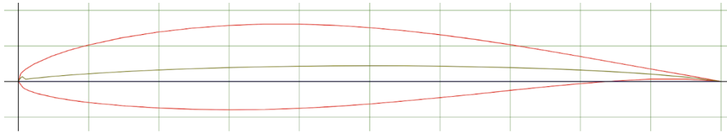
Figure 7: Cross-sectional view of root NACA 63-415 (top) and tip NACA 63-412 (bottom)
