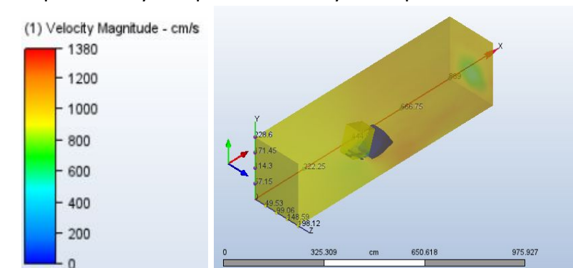
Figure 19: CFD Analysis Without Fairing
