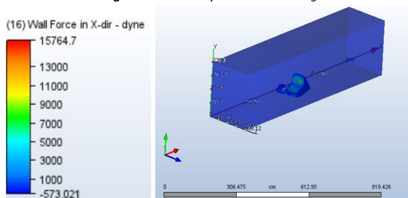
Figure 19: CFD Analysis Without Fairing
