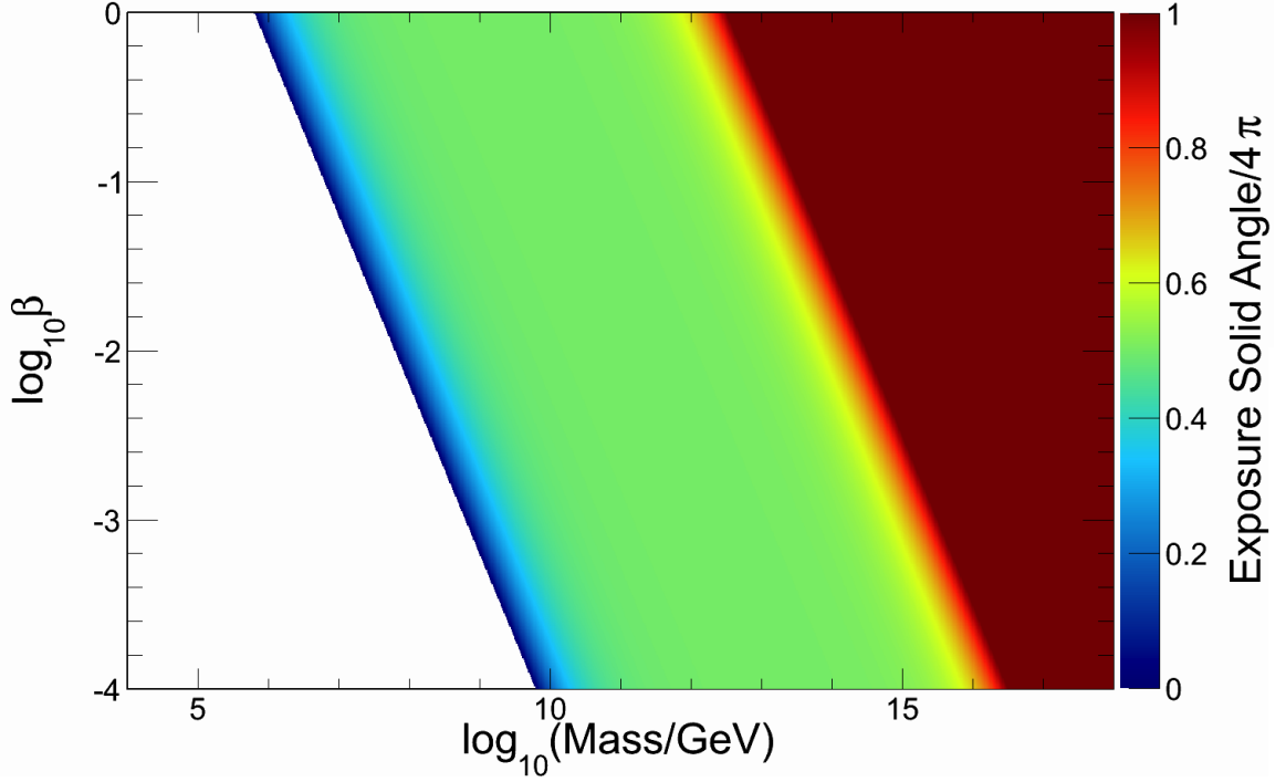
Figure 1.10: The magnetic monopole solid angle acceptance of the NO \nu A far detector as a function of monopole mass and velocity. We have assumed monopoles of a single Dirac charge ( g_D ) and no additional electronic charge.
