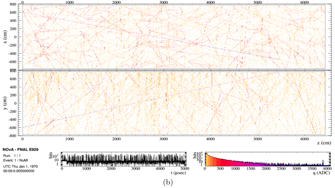
Figure 3.1: The event display shows the energy and time response of all the channels in both horizontal (y) and vertical (x) planes. Each hit is colored based on its DCS value in units of ADC counts, representing the uncalibrated energy deposit. (a) The event display of a simulated nonrelativistic ( \beta \sim 10^{-2} ) monopole's trajectory in both XZ and YZ views, with noise hits. (b) The same simulated monopole event overlaid with 5 ms of simulated cosmic-ray hits and noise hits.
