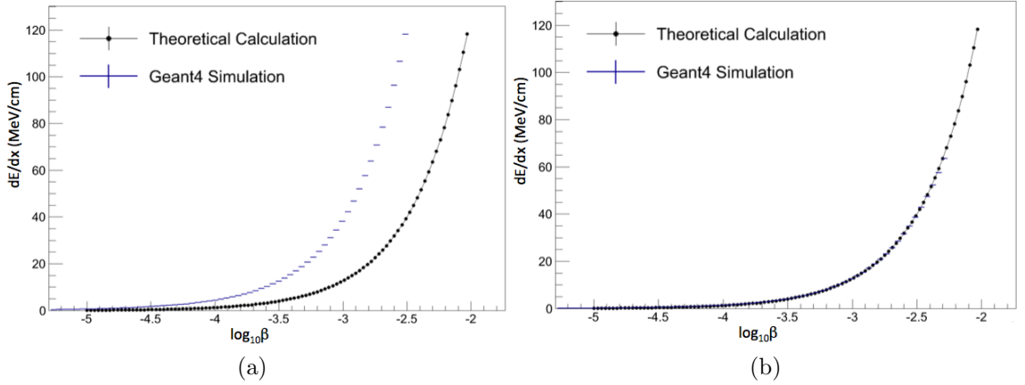
Figure 3.8: Comparison of the theoretical prediction and simulation of the slow monopole energy loss vs \beta . We see the discrepancy in the (a) simulated result of Geant 4.9.5 without correction, and (b) the correction to Geant4 discussed in the text.
