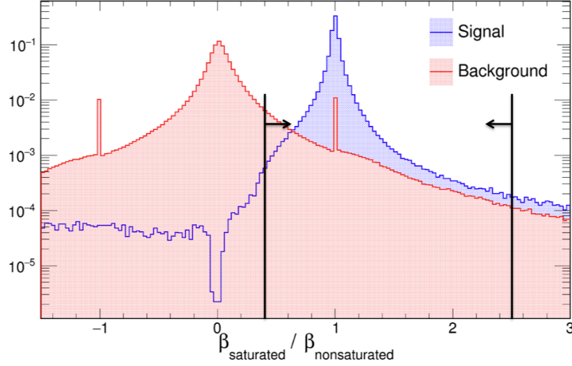
Figure 6.12: The \beta_{sat}/\beta_{nonsat} distribution of signal (blue) and background (red) events after after preselection cuts 1 and 2. The consistency check of the velocity validation cuts requires the value of \beta_{sat}/\beta_{nonsat} to be within (0.4,2.5) (black arrows).
