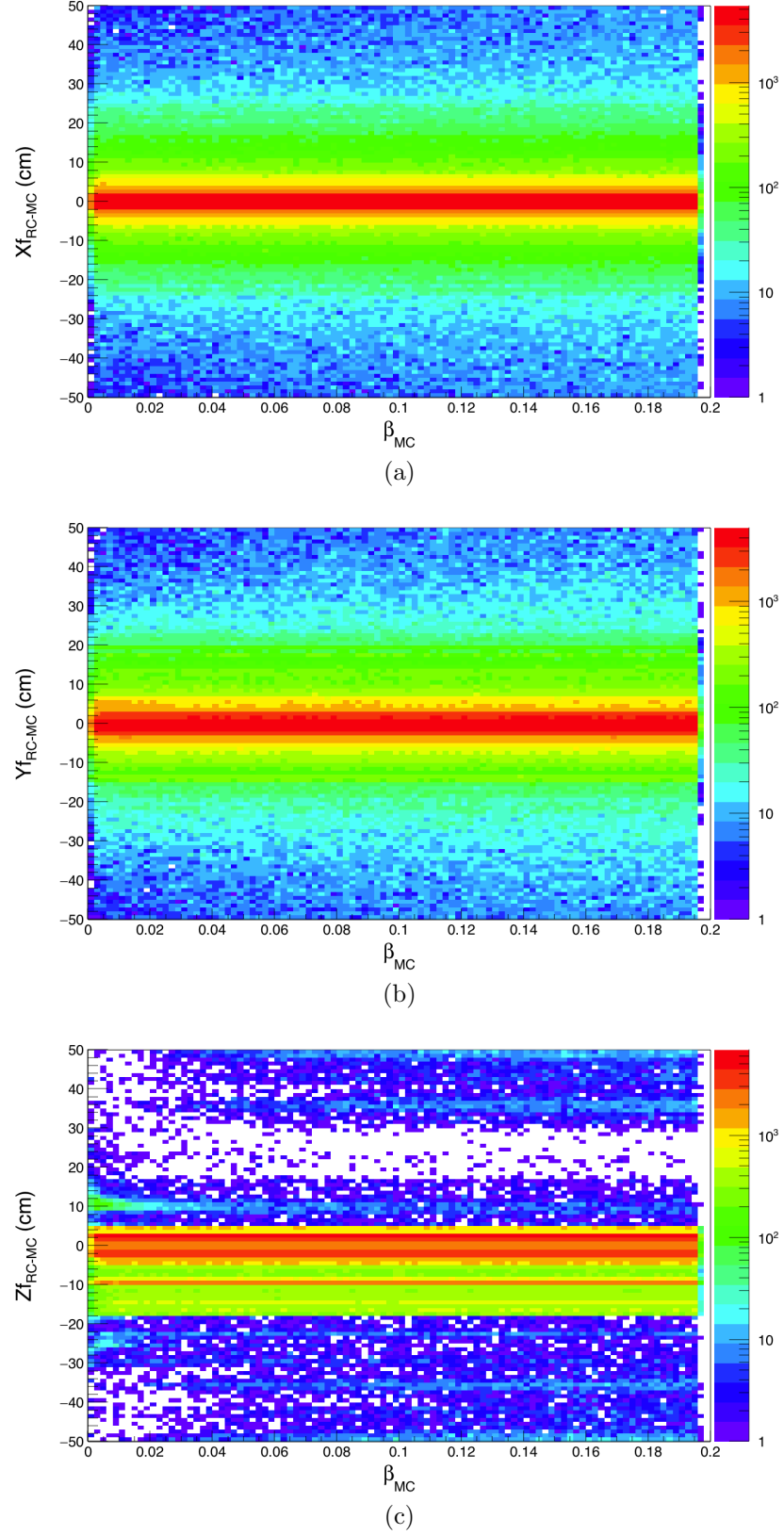
Figure 5.8: Monte Carlo test of the monopole track exit position reconstruction. The distance between the x, y, z components of the reconstructed and true exit position of the simulated monopole, is given respectively in (a), (b), and (c).
