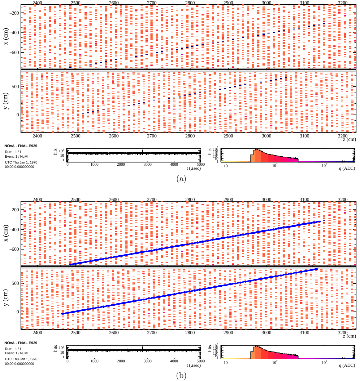
Figure 5.1: Illustration of how the offline monopole track reconstruction finds hits associated with a simulated monopole. A simulated monopole ( \beta = 0.1 ) track overlaid with simulated noise hits is shown in (a). All the hits associated with the reconstructed track are highlighted in blue as shown in (b).
