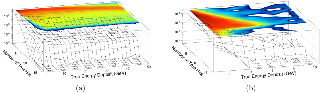
Figure 4.9: Total energy and number of hits for monopole events that fail (a) the fast ( \beta > 0.01 ) and (b) slow ( 10^{-4} < \beta < 0.01 ) monopole slicing. The plots have been normalized to one. The same slicer was used in both cases.
