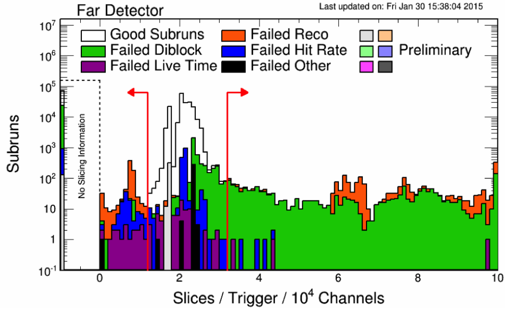
Figure 6.2: Typical distribution of the slices per subrun. Subruns in the region where the red arrows point to fail the data quality cuts. Trigger here stands for the pulser trigger which collects minimum-bias data.
