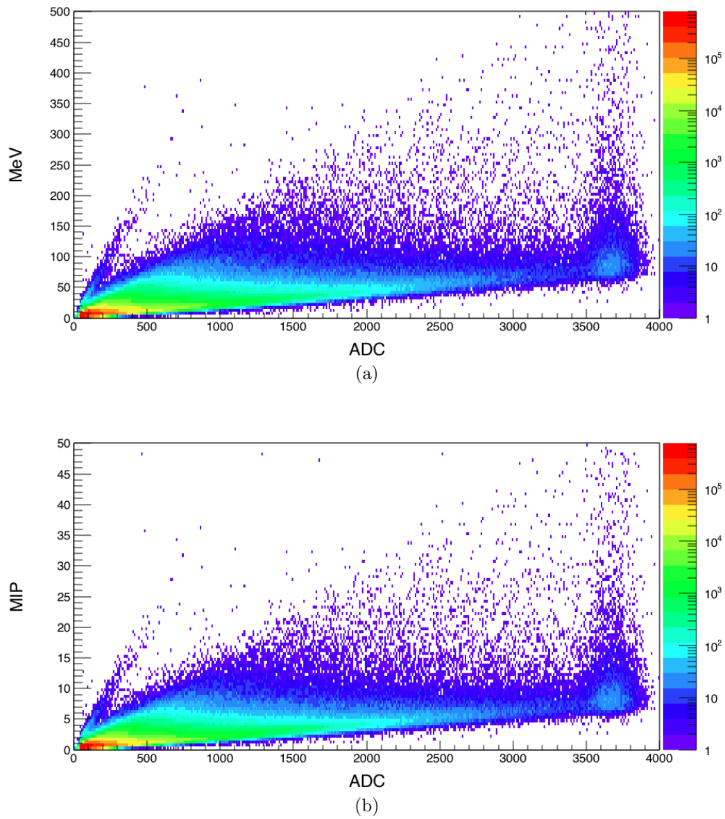
Figure 2.16: The calibrated energy deposit in a cell vs. DCS value in ADC, in the units of (a) MeV and (b) MIP.
