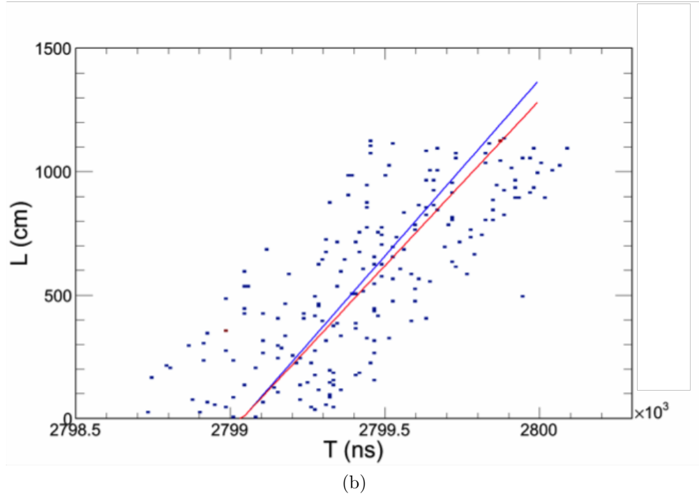
Figure 5.3: Example of reconstructing a Monte Carlo monopole velocity. (a) The event display of the reconstructed Monte Carlo monopole ( \beta = 0.045 ) track. Hits not associated with the reconstructed track have been dimmed. (b) A scatterplot of the distance vs. time of the reconstructed track points shown in (a). The slope of the red line corresponds to the true velocity of 1.34 cm/ns, and the slope of the blue line corresponds to the best fit velocity of 1.43 cm/ns.
