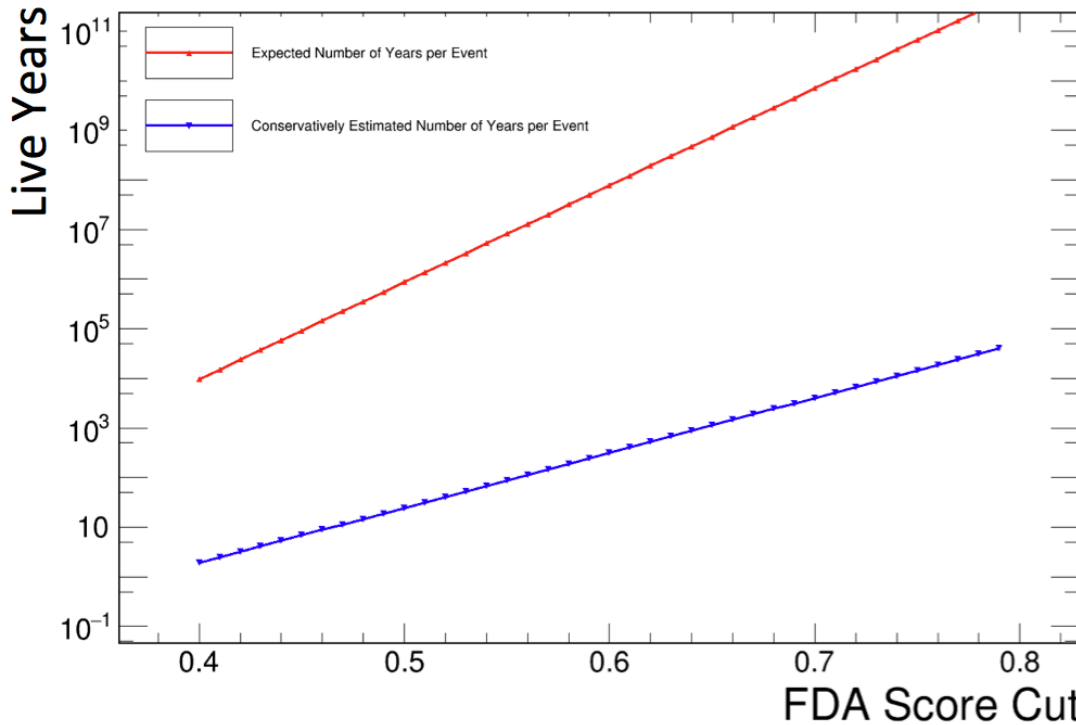
Figure 6.29: The FDA background predictions, in live years per event, in the NO \nu A far detector for the: (a) standard (given by the best fit) and (b) conservative estimates.
