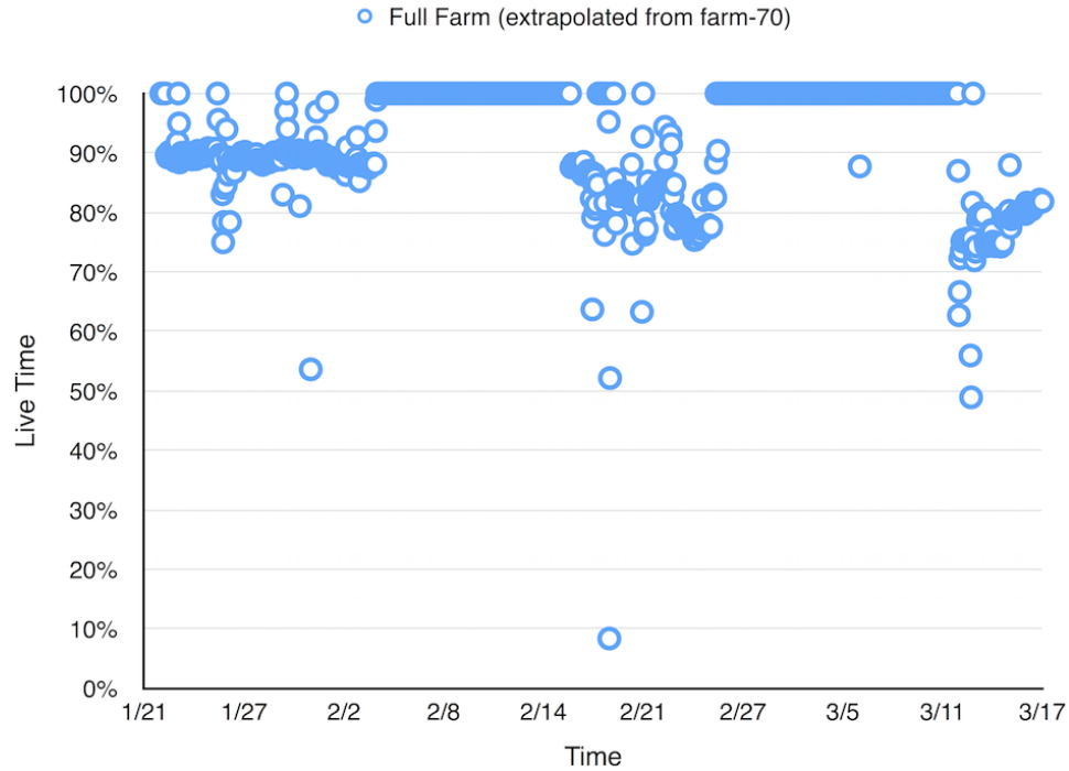
Figure 6.5: The live-time fraction from January 21 to March 16. The data is taken from one of the fastest buffer nodes (farm-70), which was implemented on January 21st, 2015.
