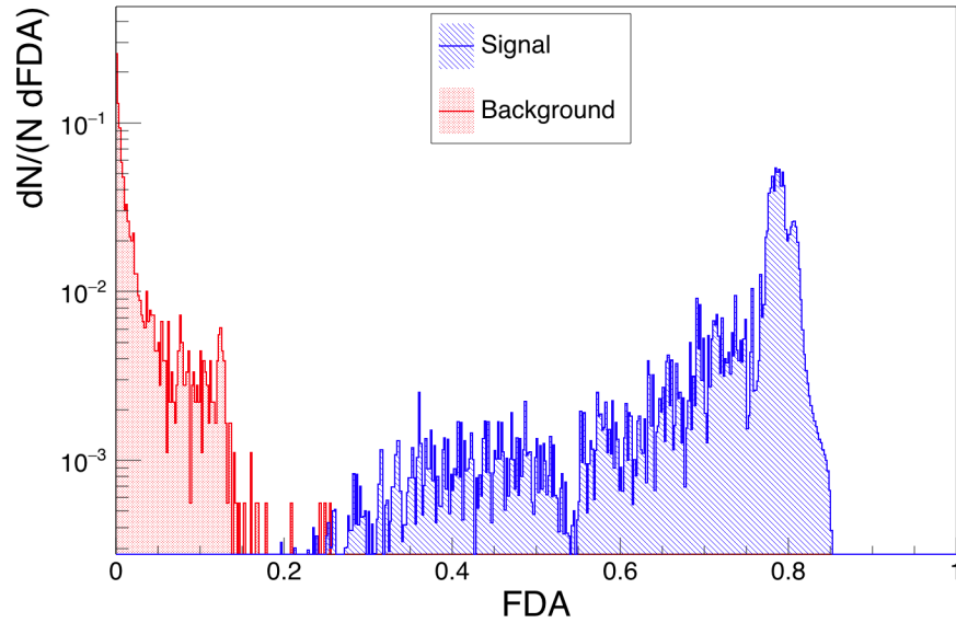
Figure 6.24: The FDA scores (with unit normalization) of signal (blue) and background (red) events, after preselection cut 1 through cut 4 (bremsstrahlung rejection cut).
