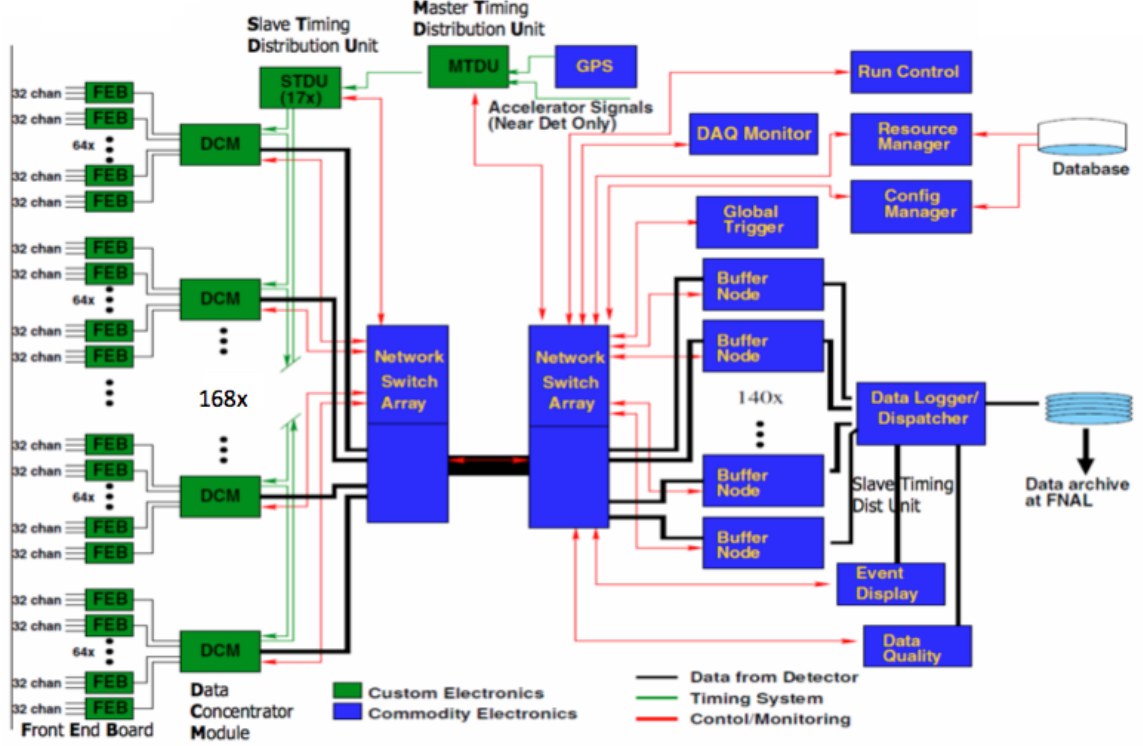
Figure 2.6: Topology of the NOνA data acquisition system.
