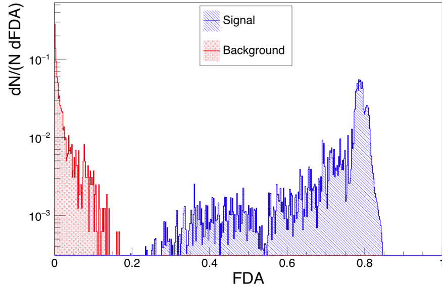
Figure 6.26: The FDA scores (with unit normalization) of signal (blue) and background (red) events, after preselection cut 1 through cut 6 (time window cut). In this plot, there is one track in the background training data set with a particularly high score of 0.17. This is a high-energy cosmic muon with bremsstrahlung. It is rejected by the last preselection cut (penetration cut).
