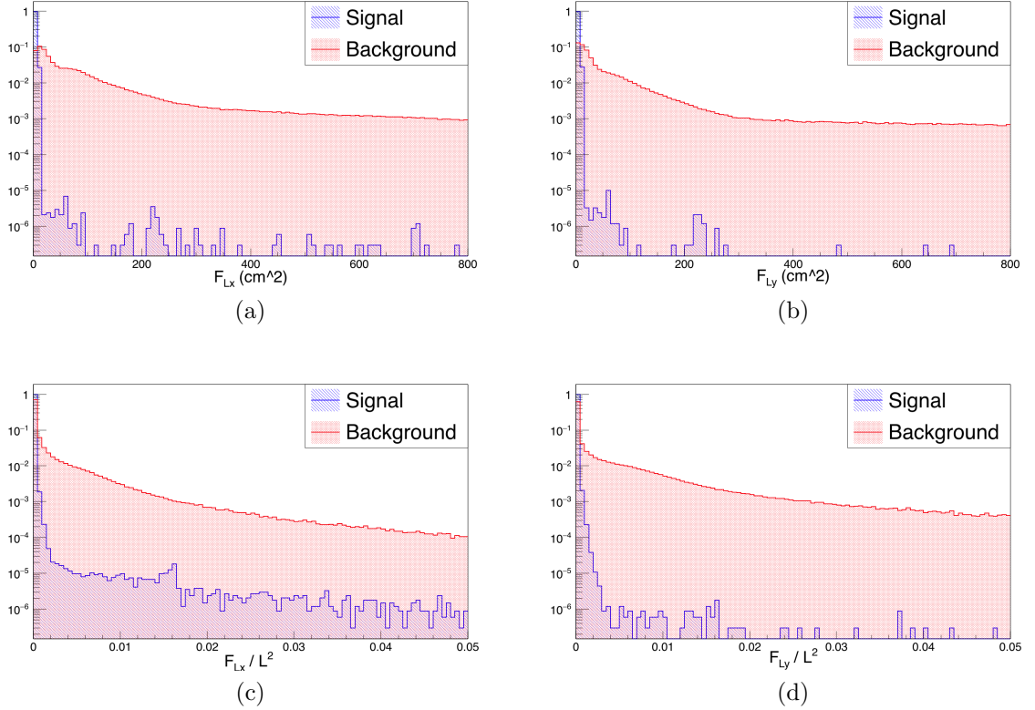
Figure 6.9: The distribution (after preselection cut 1) of track fatness F_L in the (a) X view and the (b) Y view, as well as the distribution of fractional track fatness F_L/L^2 (where L is the reconstructed track length) in the (c) X view and the (d) Y view. The track fatness cuts reject track with F_L > 15 \text{ cm}^2 or F_L/L^2 > 0.001 in either the X or Y views.
