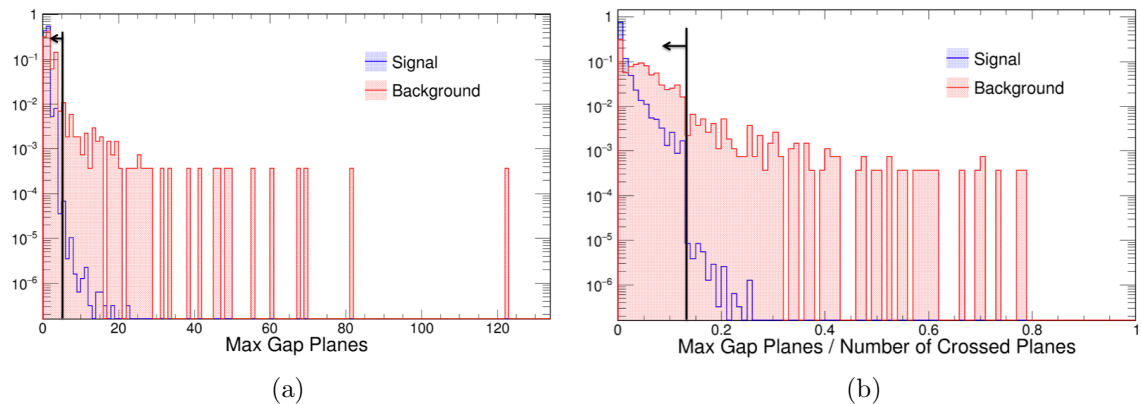
Figure 6.16: The distribution of the maximum gap in the number of missing planes (a) and gap ratio (b), for signal (blue) and background (red) events after preselection cuts 1 through 4. The maximum gap cut require the maximum gap to be less than 6 planes, and the gap ratio to be no more than 13%.
