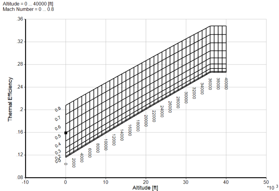
Figure 32: Parametric Analysis, Altitude and Mach Number vs. Thermal Efficiency
