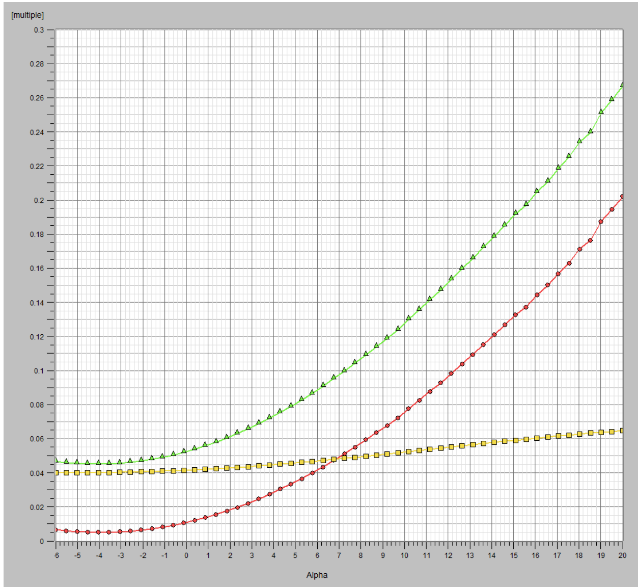
Figure 16: CD For -6° to 20° AoA
