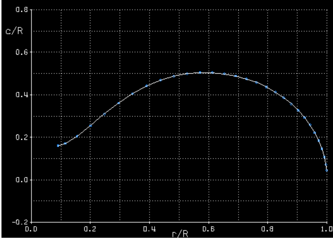
Figure 47: Final Rotor Model Chord Distribution (c/R vs r/R)
