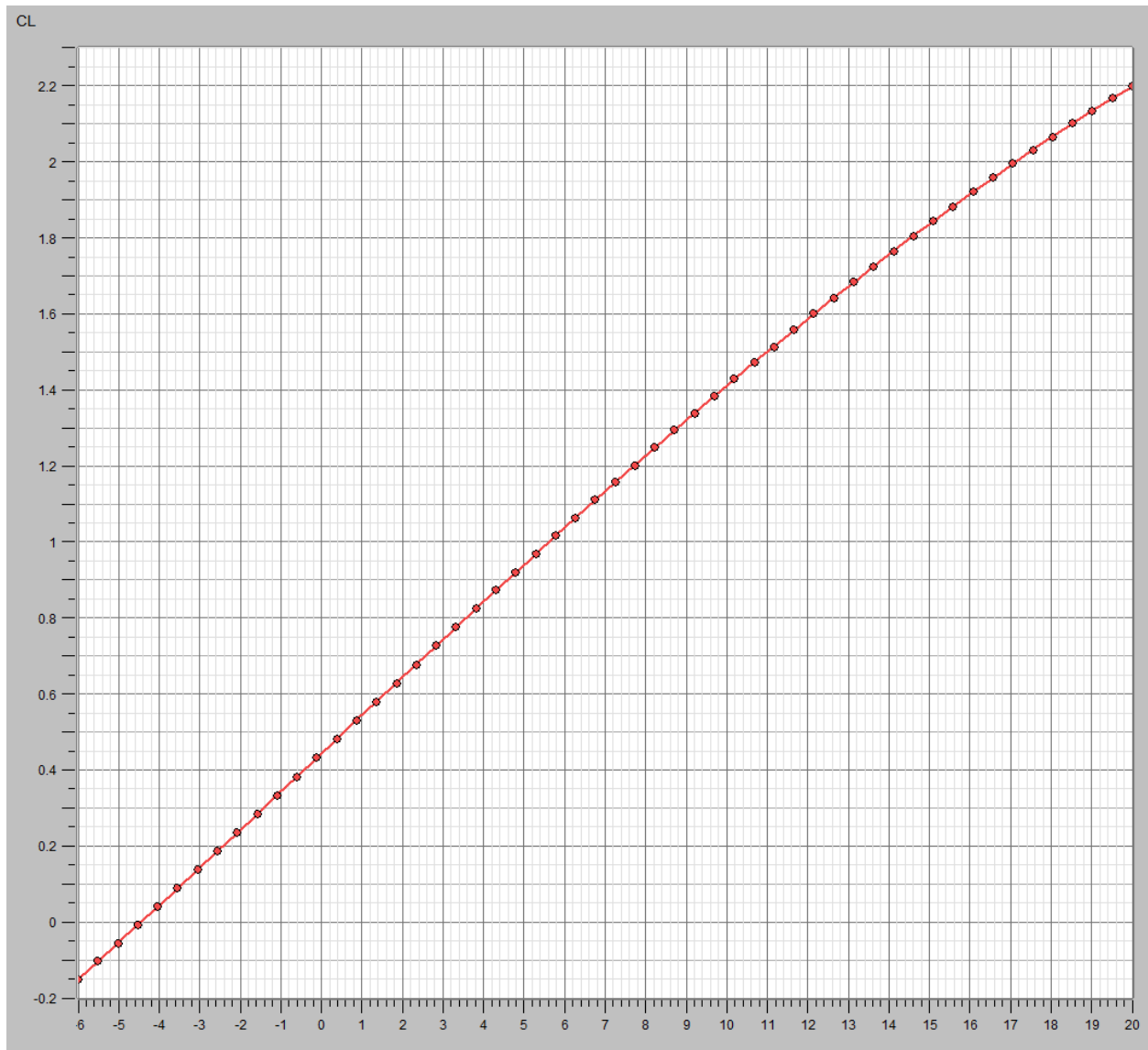
Figure 15: CL For -6^{\circ} to 20^{\circ} AoA
