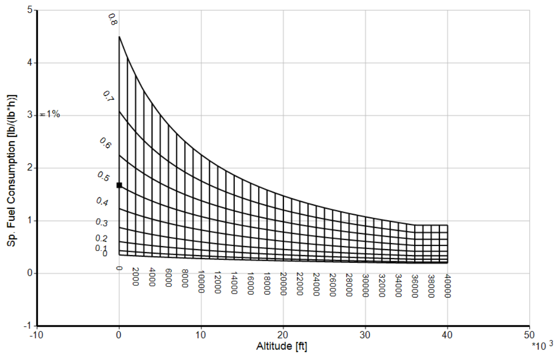
Figure 31: Parametric Analysis, Altitude and Mach Number vs. Thrust Specific Fuel Consumption
