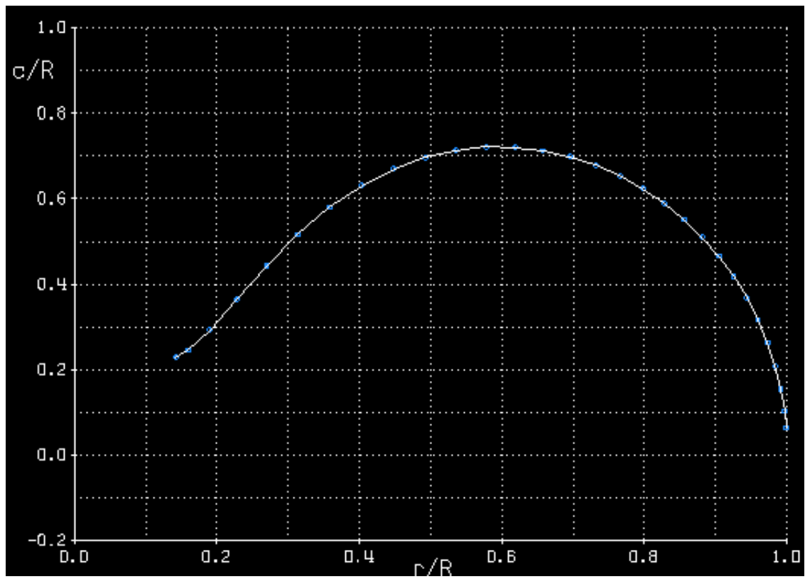
Figure 45: Initial Rotor Model Chord Distribution ( c/R vs r/R )
