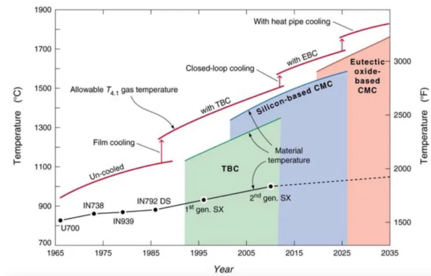
Figure 35: Expected Future Engine Temperature Capabilities [8]
