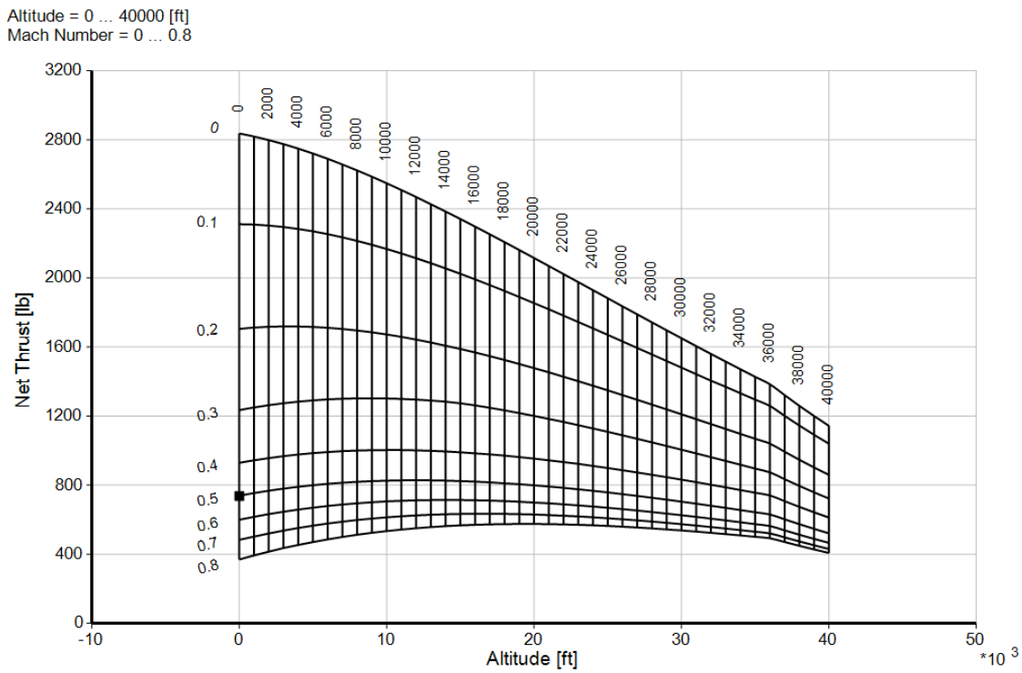
Figure 30: Parametric Analysis, Altitude and Mach Number vs. Net Thrust
