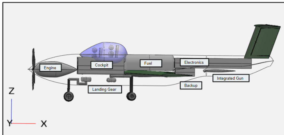
Figure 10: Cross-Section Side View of Final Aircraft In OpenVSP, Major Components Shown
