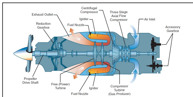
Figure 22: Reverse Flow Turboprop [2]
