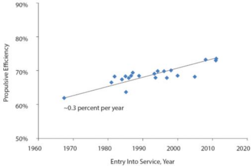
Figure 37: A Trend of Engine Propulsive Efficiency Improvements By Year [9]
