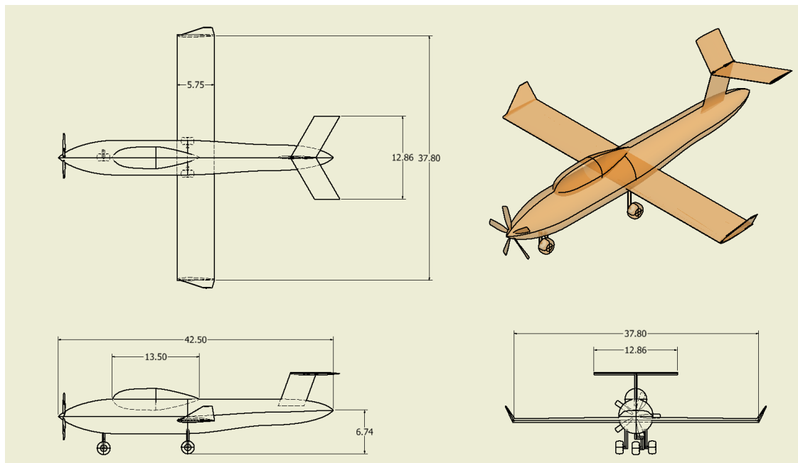
Figure 8: Isometric View of Initial Aircraft In Solidworks
