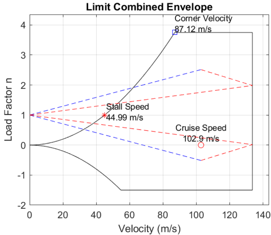
Figure 56: V-n Diagram with Gust Lines With ULF = 4
