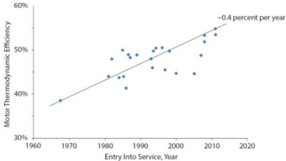
Figure 36: A Trend of Engine Thermodynamic Efficiency Improvements By Year [9]
