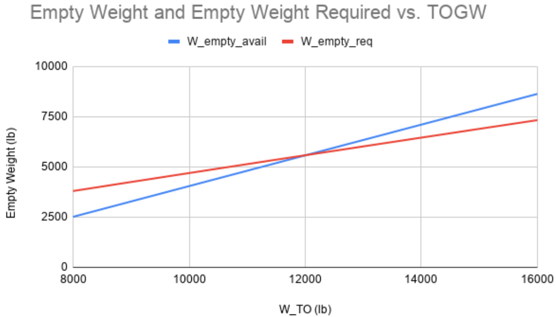
Figure 7: Empty Weight Calculations as a Function of TOGW
