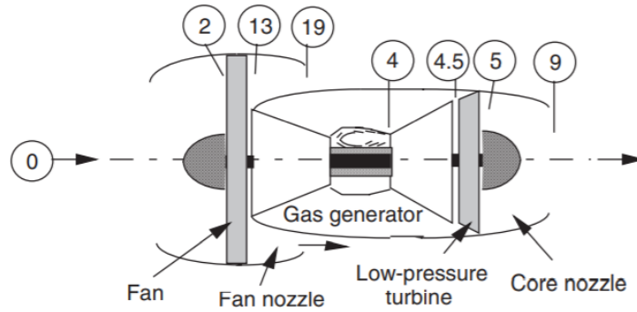
Figure 24: Separate Exhaust Turbofan Engine Schematic [3]
