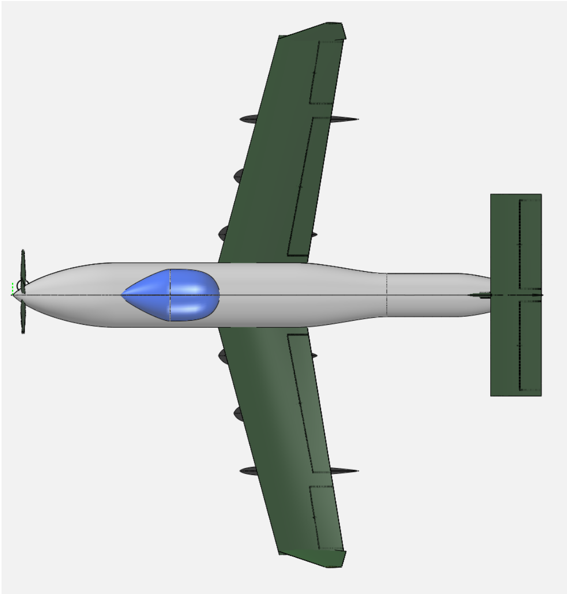
Figure 17: Final Wing Design
