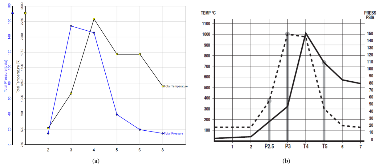
Figure 28: Total Temperature and Pressure Graphs By Engine Stage (Left: GasTurb, Right: PT-6A manual)
