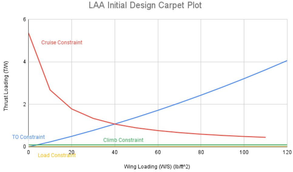
Figure 6: Carpet Plot
