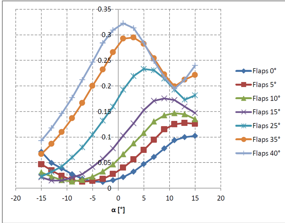
Figure 20: NACA 63A-415 with Flaps C_D Curve [1]
