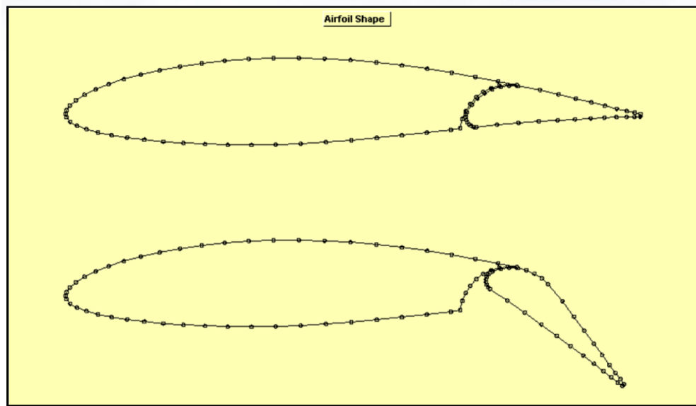
Figure 18: NACA 63A-415 with Single Slotted Flaps Geometry [1]
