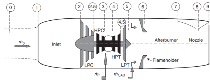
Figure 23: Afterburning Turbojet Engine Schematic [3]
