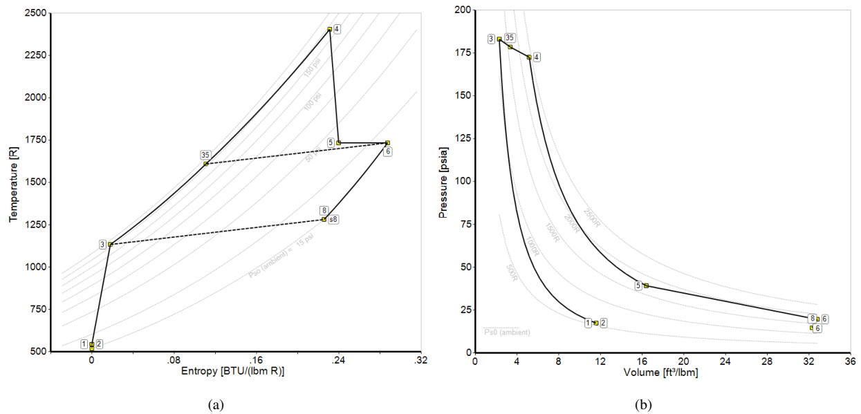
Figure 38: T-S and P-V Diagrams
