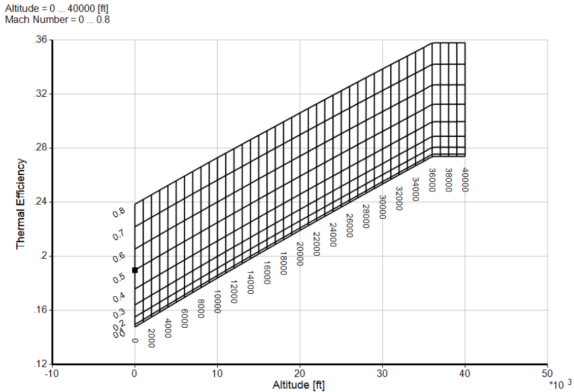
Figure 43: Parametric Analysis, Altitude and Mach Number vs. Thermal Efficiency
