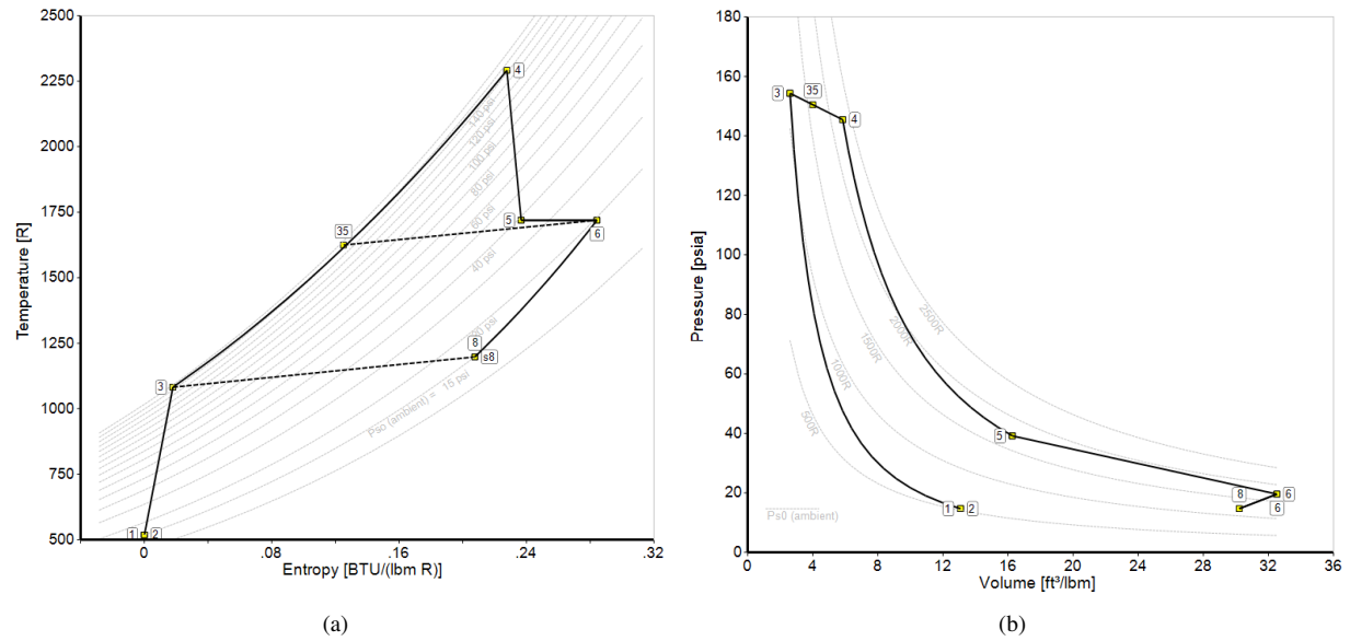
Figure 27: T-S and P-V Diagrams
