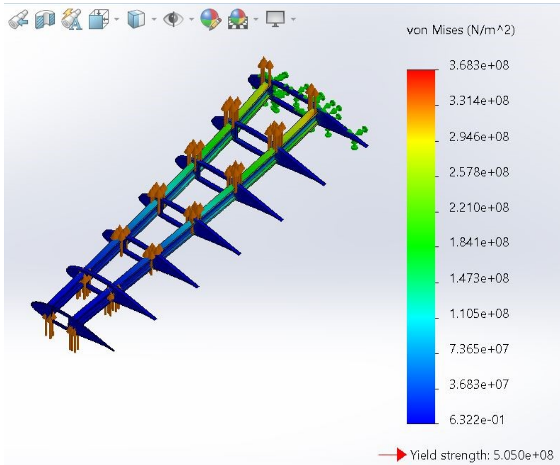
Figure 54: FEA of the Wing
