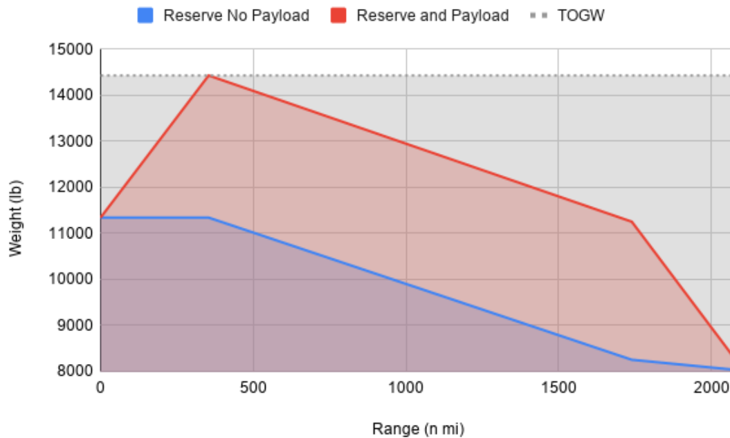
Figure 59: Payload Range Diagram. Note that the bottom of the chart is set at the OEW
