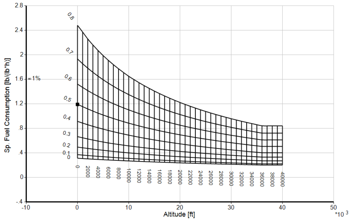
Figure 41: Parametric Analysis, Altitude and Mach Number vs. Net Thrust
