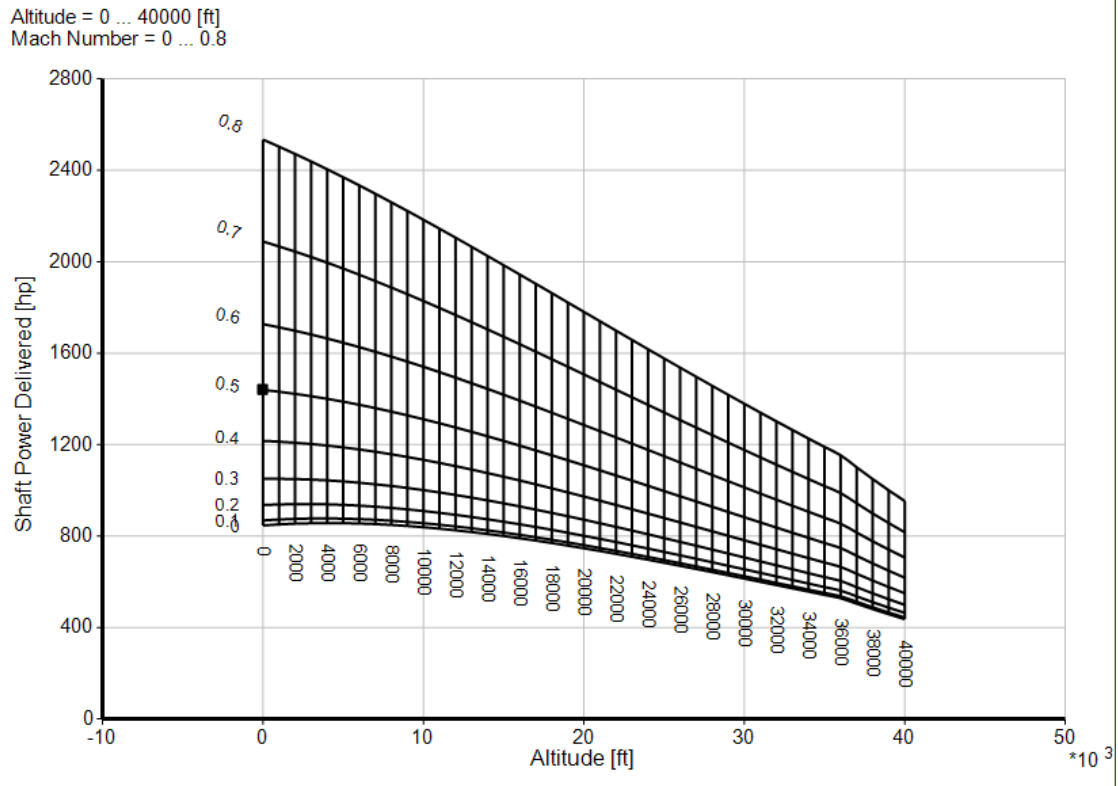
Figure 29: Parametric Analysis, Altitude and Mach Number vs. Shaft Power Delivered
