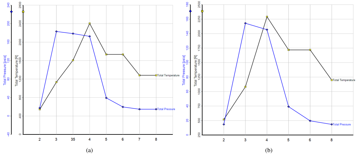
Figure 39: Total Temperature and Pressure Graphs By Engine Stage (Left: 2025 PT-6A GasTurb, Right: Current PT-6A GasTurb)
