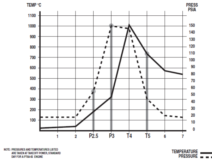
Figure 26: PT-6A Total Temperatures and Pressures By Engine Stage [5]
