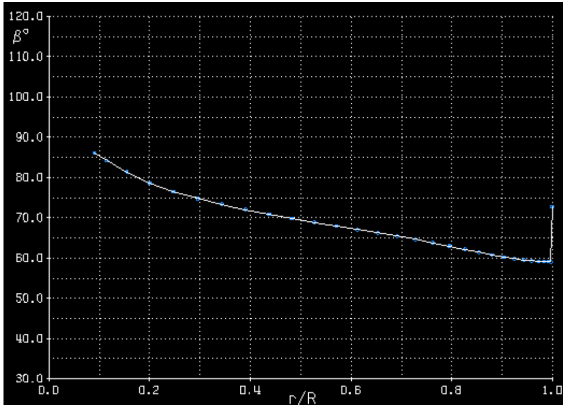
Figure 48: Final Rotor Model Blade Twist Angle Distribution ( \beta_0 vs r/R )
