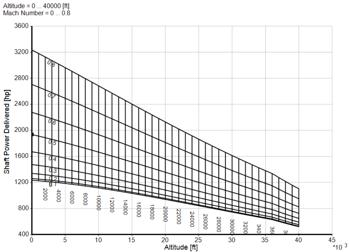
Figure 40: Parametric Analysis, Altitude and Mach Number vs. Shaft Power Delivered
