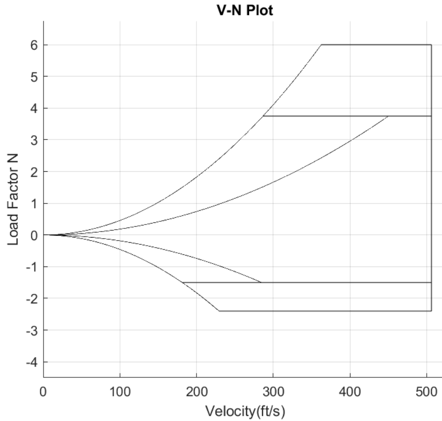
Figure 55: V-n Diagram
