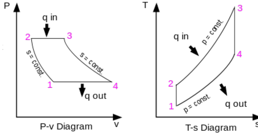
Figure 33: The Brayton Cycle [6]
