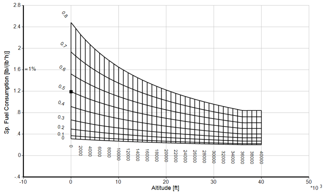
Figure 42: Parametric Analysis, Altitude and Mach Number vs. Thrust Specific Fuel Consumption
