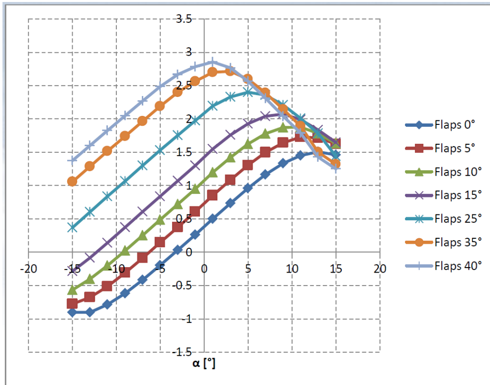
Figure 19: NACA 63A-415 with Flaps C_L Curve [1]
