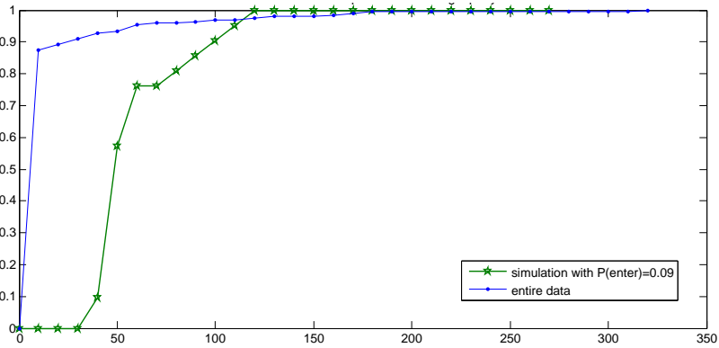
Figure 1.3: The simulated CDF of the number of people entering a party
