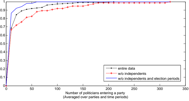
Figure 1.2: The CDF of the number of MPs entering a party
