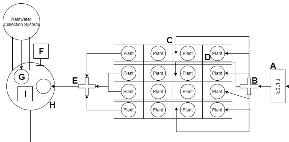
Fig. 2. Top View of Hydroponic System
