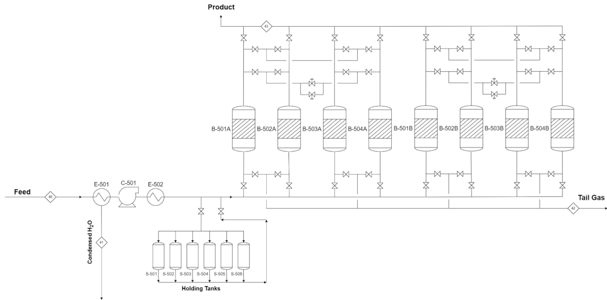
Figure 4.7-1 PFD of PSA unit
