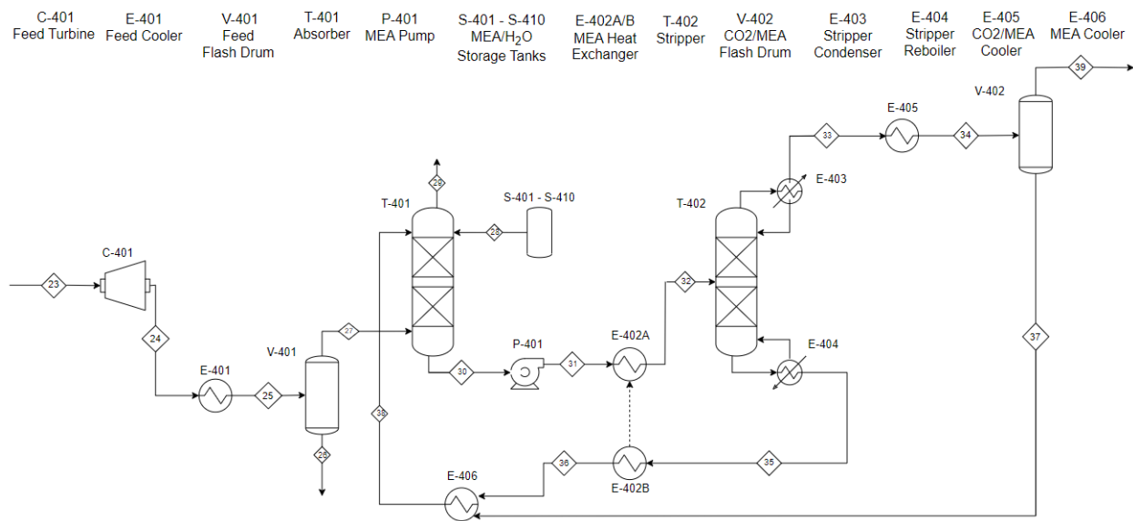
Figure 4.6-1 PFD of amine scrubber for carbon dioxide separation
