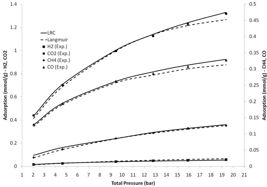
Figure 5.5-1 Equilibrium isotherms and amount of gas adsorbed on zeolite 5A at 45°C (Yavary et al., 2016)
