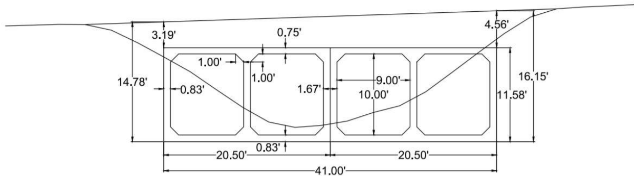
Figure 8: CAD drawing of our two twin cell box culvert system with dimensions. The sloped straight line on the top represents the roadway. The U-shaped section represents the elevation profile of the streambed.
