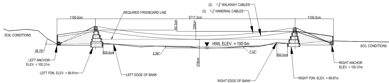
Figure 4.2.3. Design #1 Non-Standard Geometric Layout.
