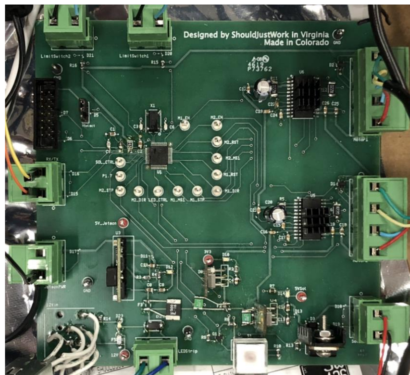
Figure 17 Soldered PCB
