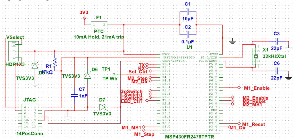
Figure 9 MSP430 Schematic
