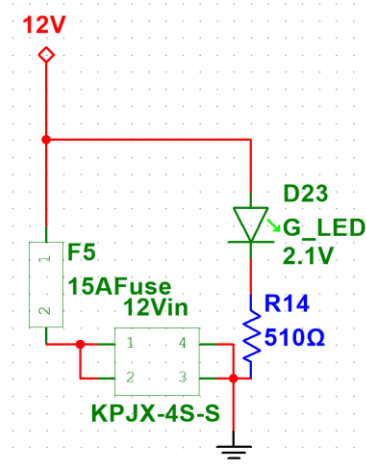
Figure 3 12V Input
